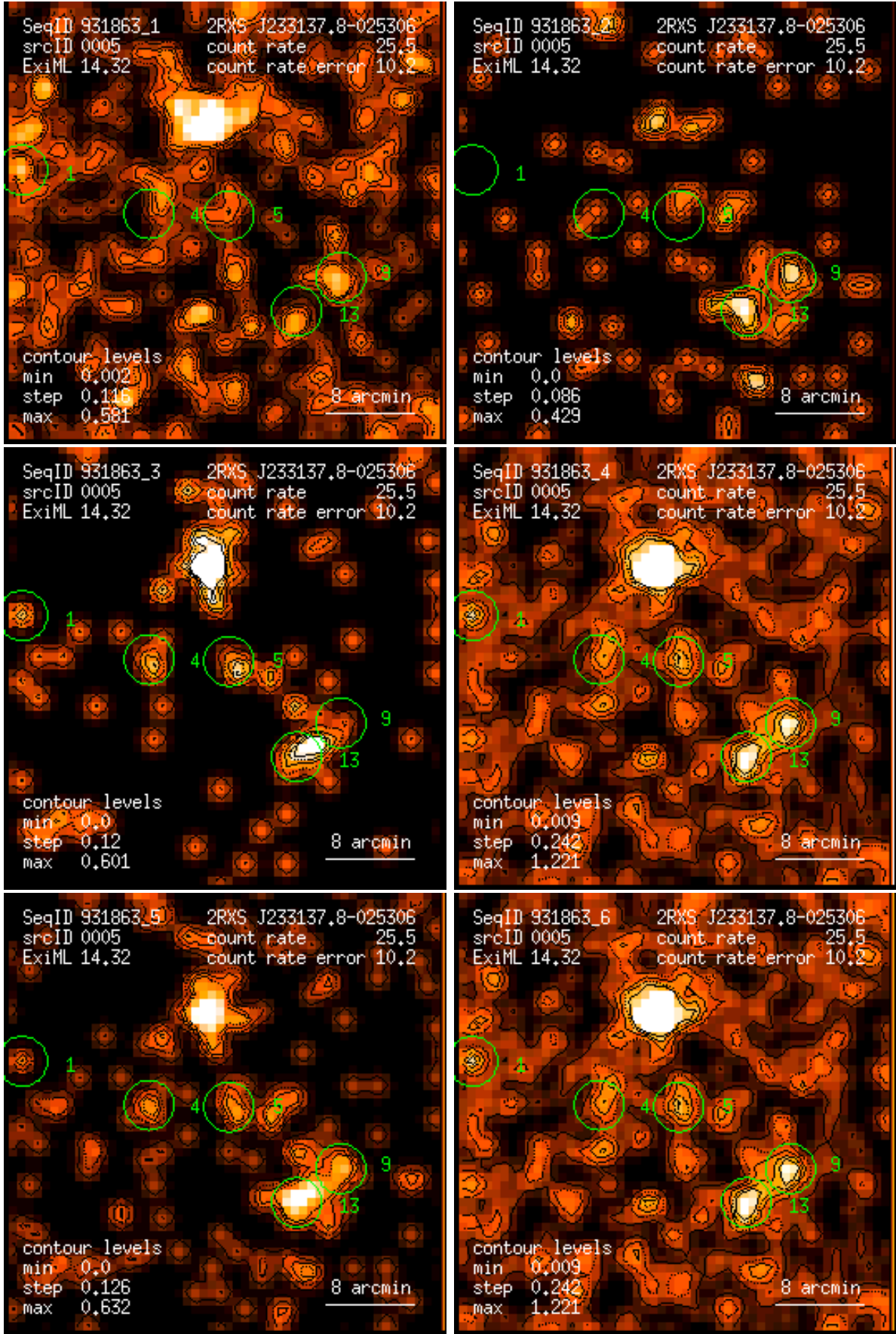
Figure 5: RASS 931863: detection 0005: band rate images, Gaussian filter: (1) PSPC channels 11 – 41, (2) 52 – 90, (3) 91 – 201, (4) 11 – 235, (5) 52 – 201, (6) 11 – 201. Broad band rates in counts/ks. Band rate contour levels in counts/ks/arcmin 2 .
