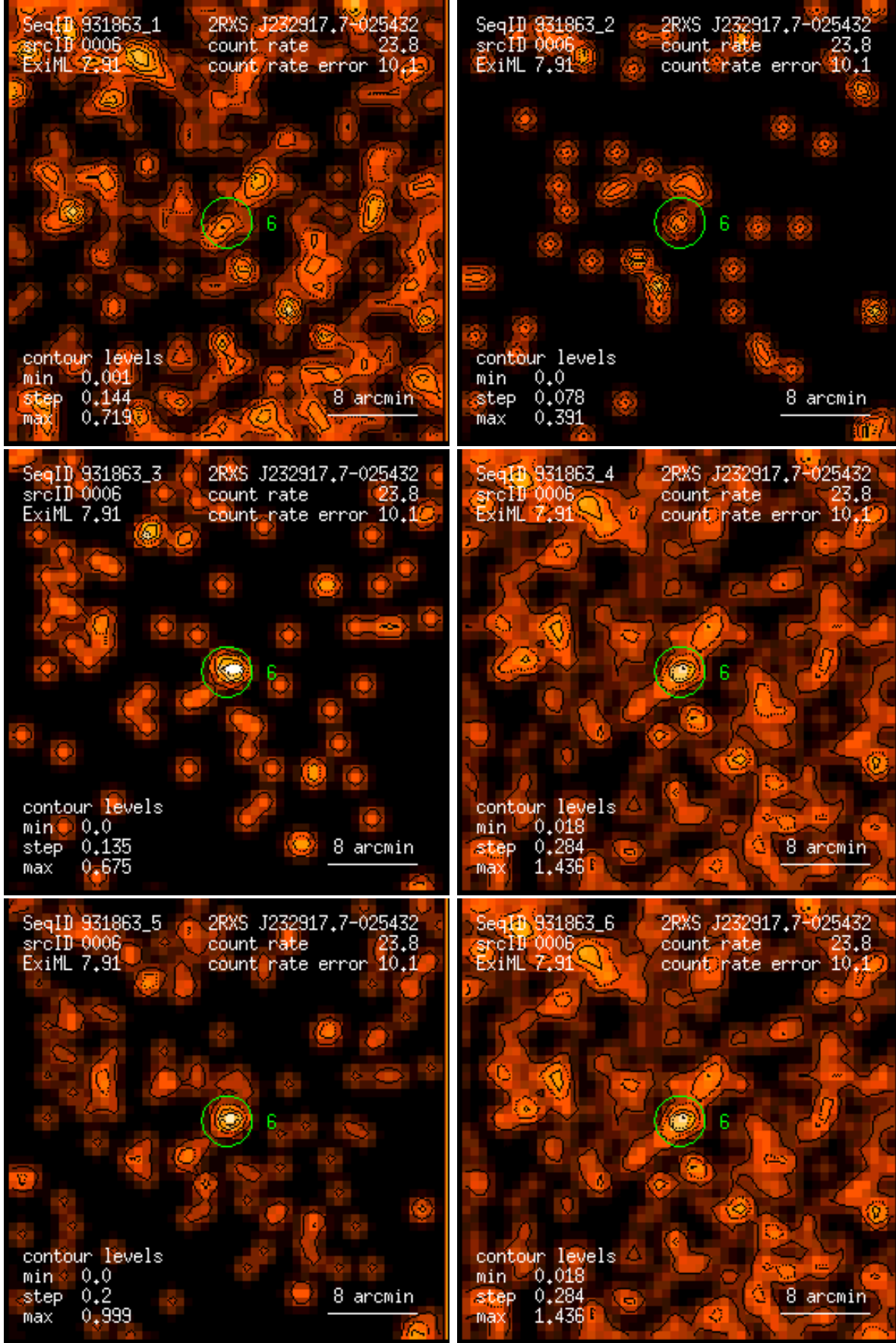
Figure 6: RASS 931863: detection 0006: band rate images, Gaussian filter: (1) PSPC channels 11 – 41, (2) 52 – 90, (3) 91 – 201, (4) 11 – 235, (5) 52 – 201, (6) 11 – 201. Broad band rates in counts/ks. Band rate contour levels in counts/ks/arcmin 2 .
