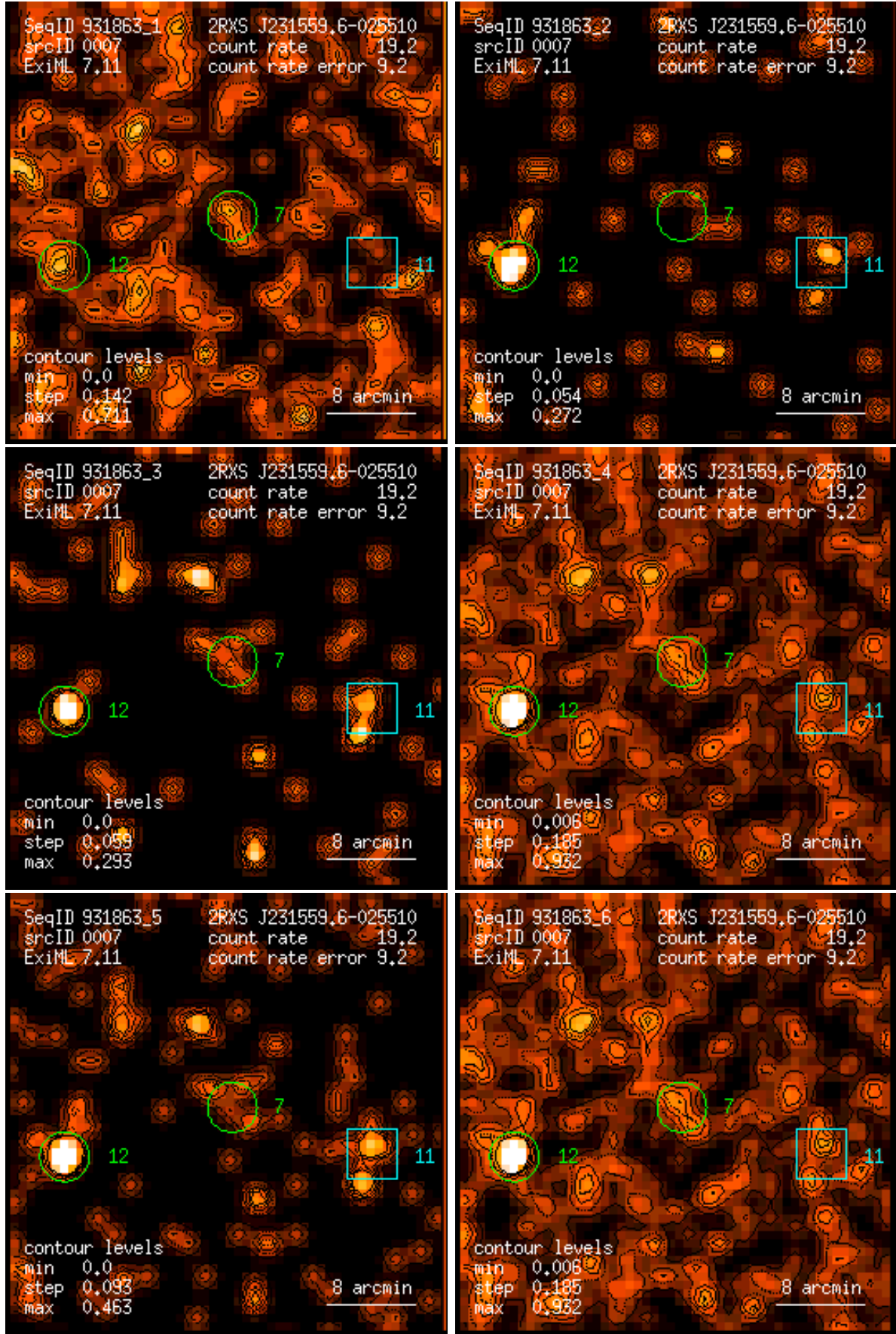
Figure 7: RASS 931863: detection 0007: band rate images, Gaussian filter: (1) PSPC channels 11 – 41, (2) 52 – 90, (3) 91 – 201, (4) 11 – 235, (5) 52 – 201, (6) 11 – 201. Broad band rates in counts/ks. Band rate contour levels in counts/ks/arcmin 2 .
