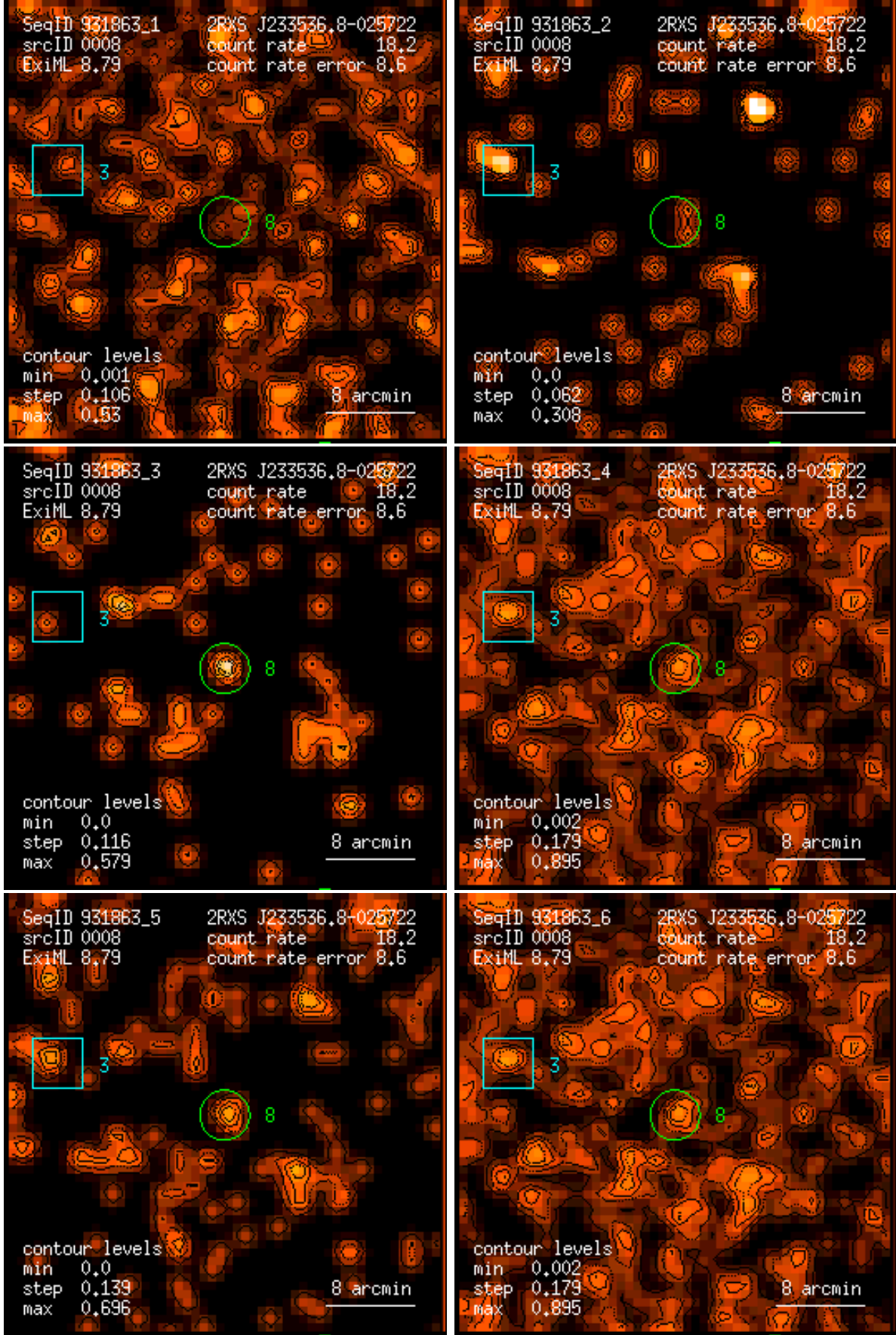
Figure 8: RASS 931863: detection 0008: band rate images, Gaussian filter: (1) PSPC channels 11 – 41, (2) 52 – 90, (3) 91 – 201, (4) 11 – 235, (5) 52 – 201, (6) 11 – 201. Broad band rates in counts/ks. Band rate contour levels in counts/ks/arcmin 2 .
