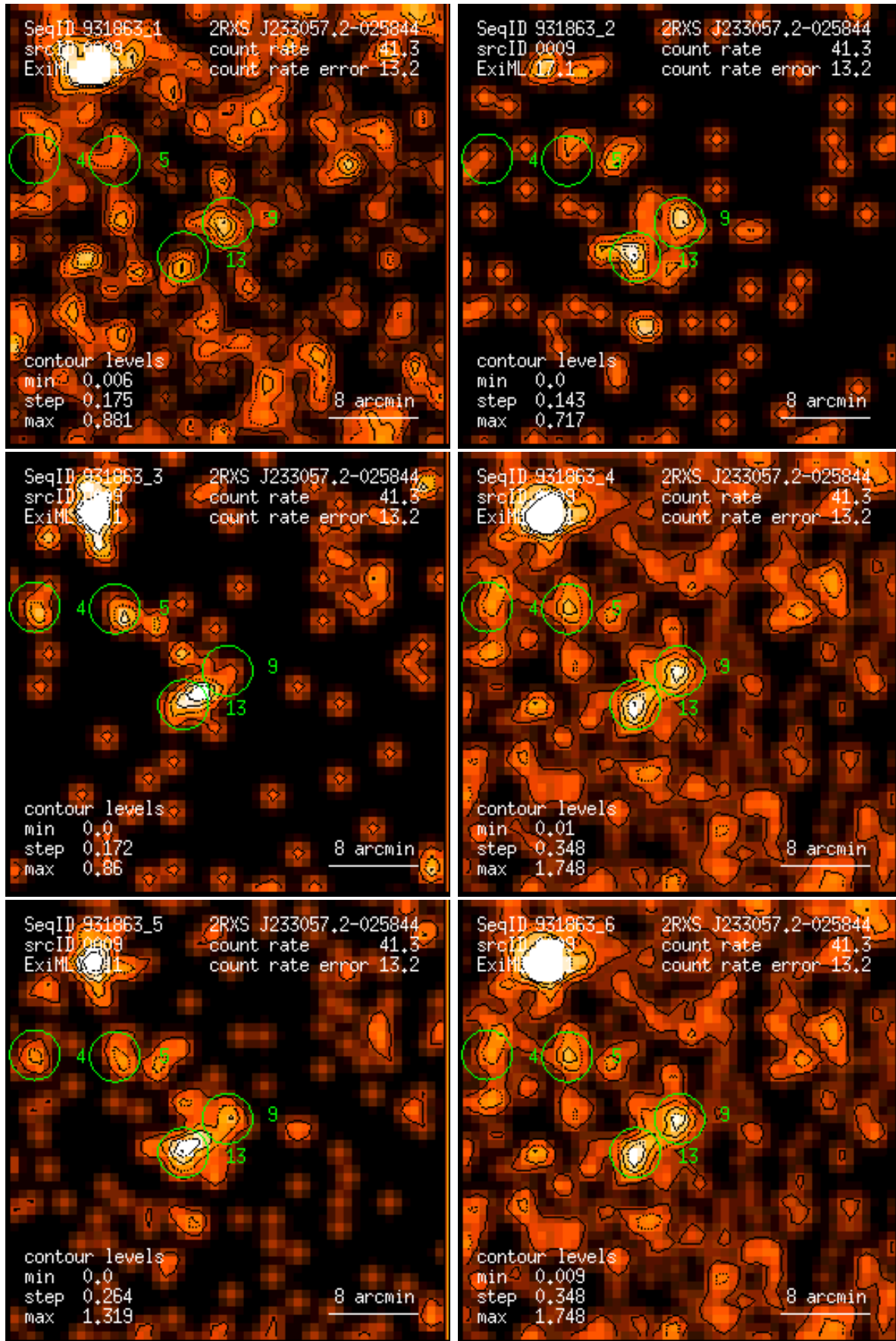
Figure 9: RASS 931863: detection 0009: band rate images, Gaussian filter: (1) PSPC channels 11 – 41, (2) 52 – 90, (3) 91 – 201, (4) 11 – 235, (5) 52 – 201, (6) 11 – 201. Broad band rates in counts/ks. Band rate contour levels in counts/ks/arcmin 2 .
