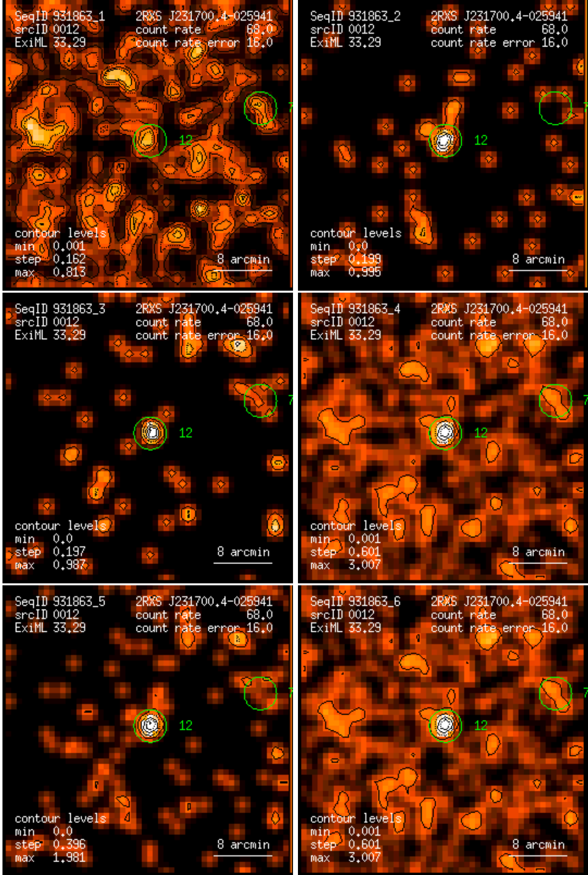
Figure 12: RASS 931863: detection 0012: band rate images, Gaussian filter: (1) PSPC channels 11 – 41, (2) 52 – 90, (3) 91 – 201, (4) 11 – 235, (5) 52 – 201, (6) 11 – 201. Broad band rates in counts/ks. Band rate contour levels in counts/ks/arcmin 2 .
