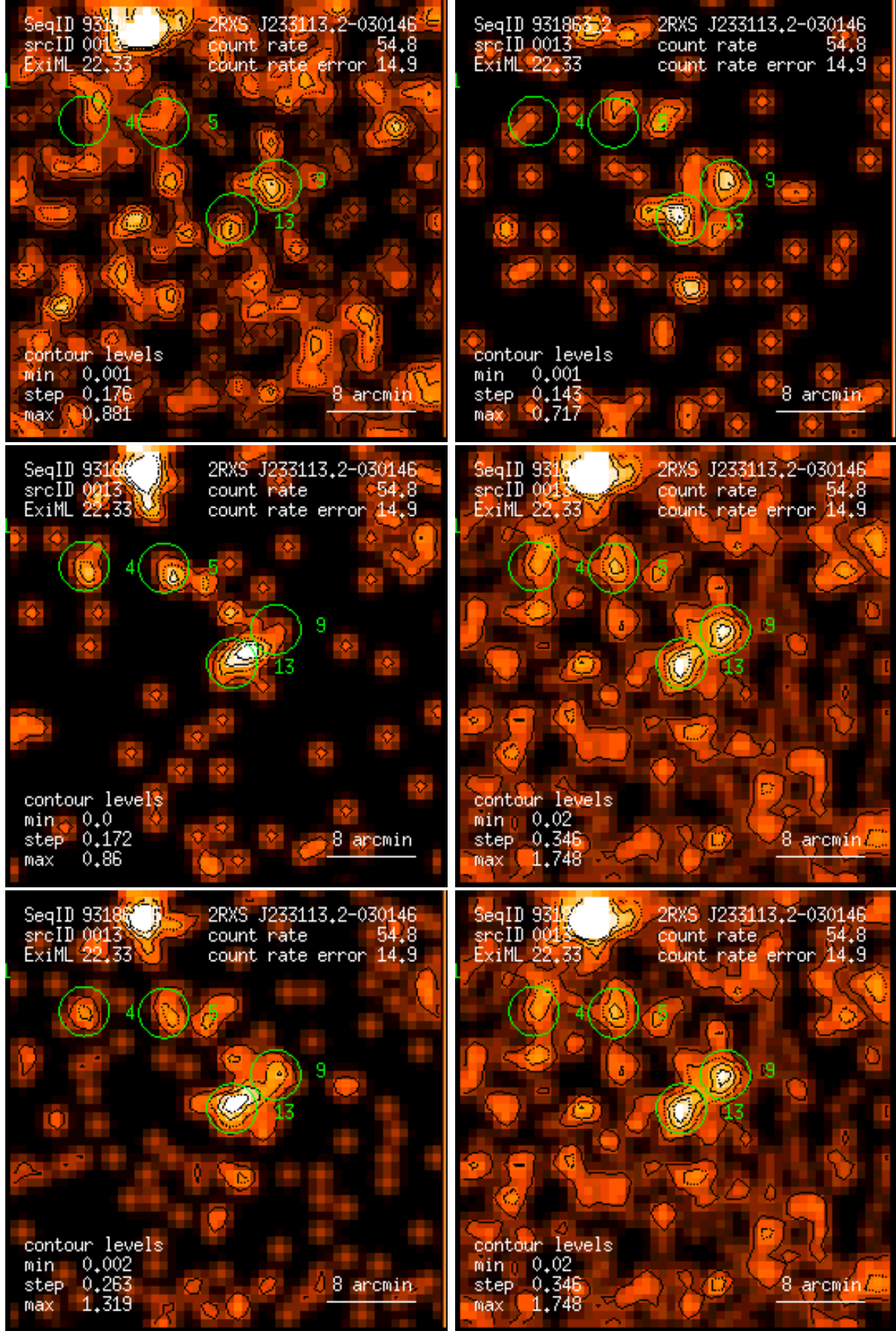
Figure 13: RASS 931863: detection 0013: band rate images, Gaussian filter: (1) PSPC channels 11 – 41, (2) 52 – 90, (3) 91 – 201, (4) 11 – 235, (5) 52 – 201, (6) 11 – 201. Broad band rates in counts/ks. Band rate contour levels in counts/ks/arcmin 2 .
