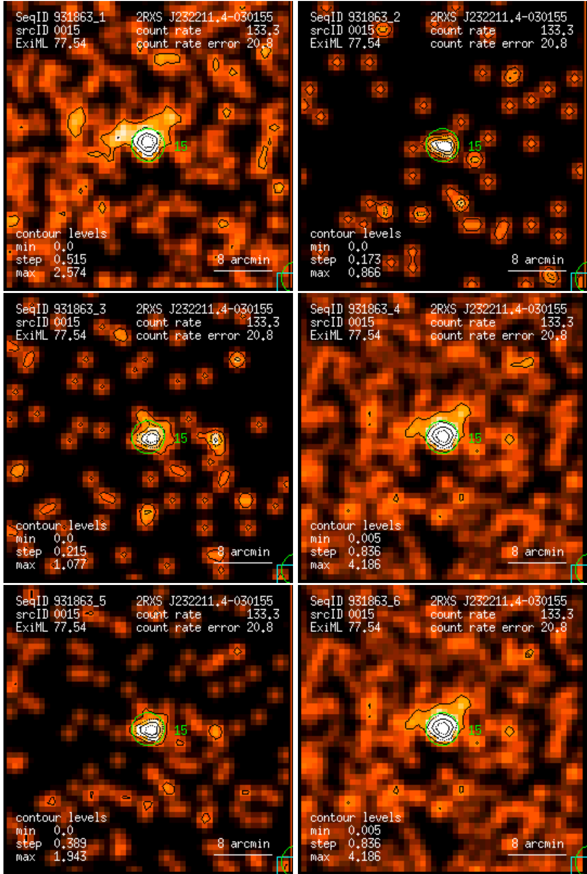
Figure 15: RASS 931863: detection 0015: band rate images, Gaussian filter: (1) PSPC channels 11 – 41, (2) 52 – 90, (3) 91 – 201, (4) 11 – 235, (5) 52 – 201, (6) 11 – 201. Broad band rates in counts/ks. Band rate contour levels in counts/ks/arcmin 2 .
