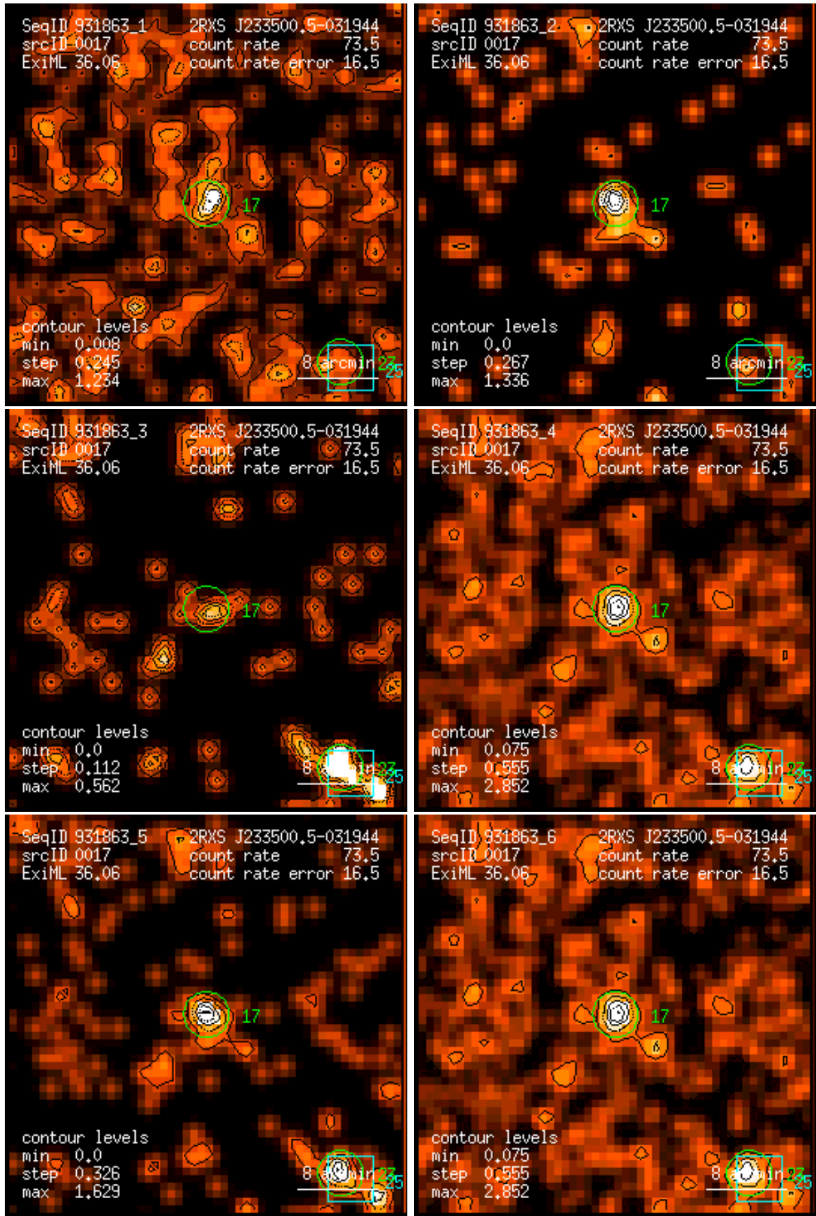
Figure 17: RASS 931863: detection 0017: band rate images, Gaussian filter: (1) PSPC channels 11 – 41, (2) 52 – 90, (3) 91 – 201, (4) 11 – 235, (5) 52 – 201, (6) 11 – 201. Broad band rates in counts/ks. Band rate contour levels in counts/ks/arcmin 2 .
