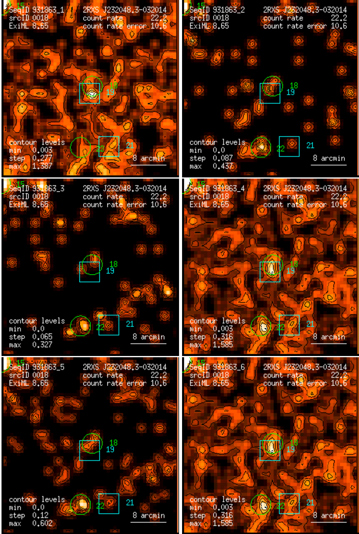
Figure 18: RASS 931863: detection 0018: band rate images, Gaussian filter: (1) PSPC channels 11 – 41, (2) 52 – 90, (3) 91 – 201, (4) 11 – 235, (5) 52 – 201, (6) 11 – 201. Broad band rates in counts/ks. Band rate contour levels in counts/ks/arcmin 2 .
