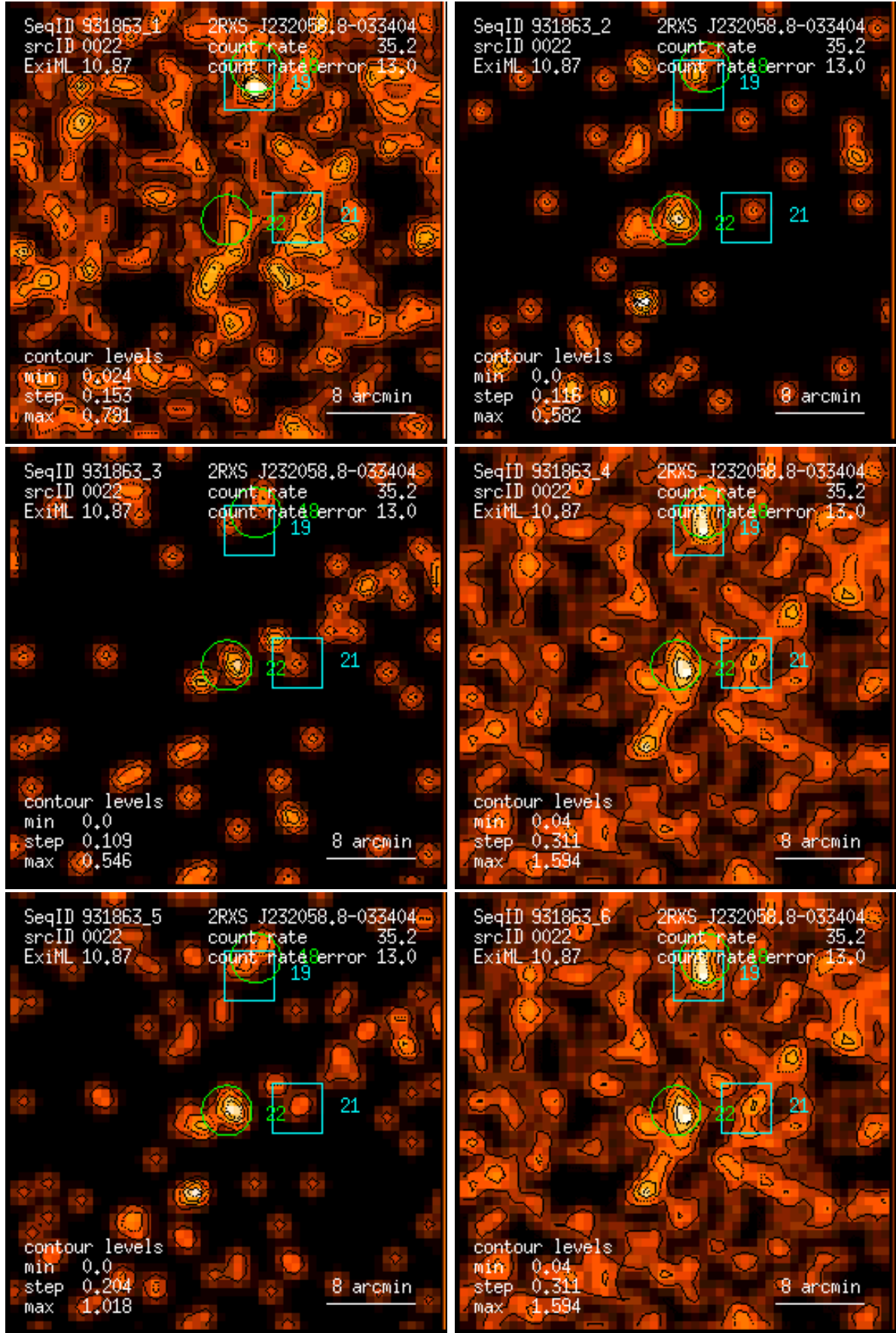
Figure 22: RASS 931863: detection 0022: band rate images, Gaussian filter: (1) PSPC channels 11 – 41, (2) 52 – 90, (3) 91 – 201, (4) 11 – 235, (5) 52 – 201, (6) 11 – 201. Broad band rates in counts/ks. Band rate contour levels in counts/ks/arcmin 2 .
