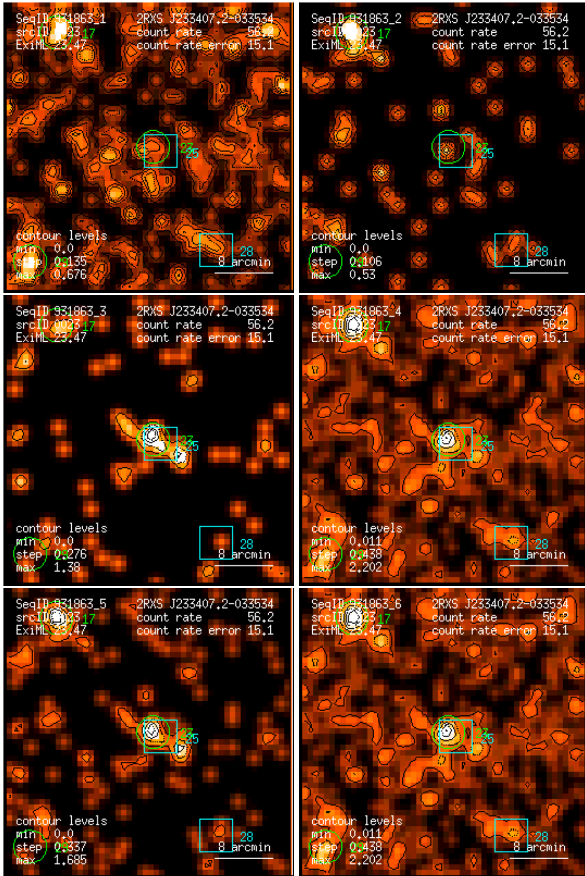
Figure 23: RASS 931863: detection 0023: band rate images, Gaussian filter: (1) PSPC channels 11 – 41, (2) 52 – 90, (3) 91 – 201, (4) 11 – 235, (5) 52 – 201, (6) 11 – 201. Broad band rates in counts/ks. Band rate contour levels in counts/ks/arcmin 2 .
