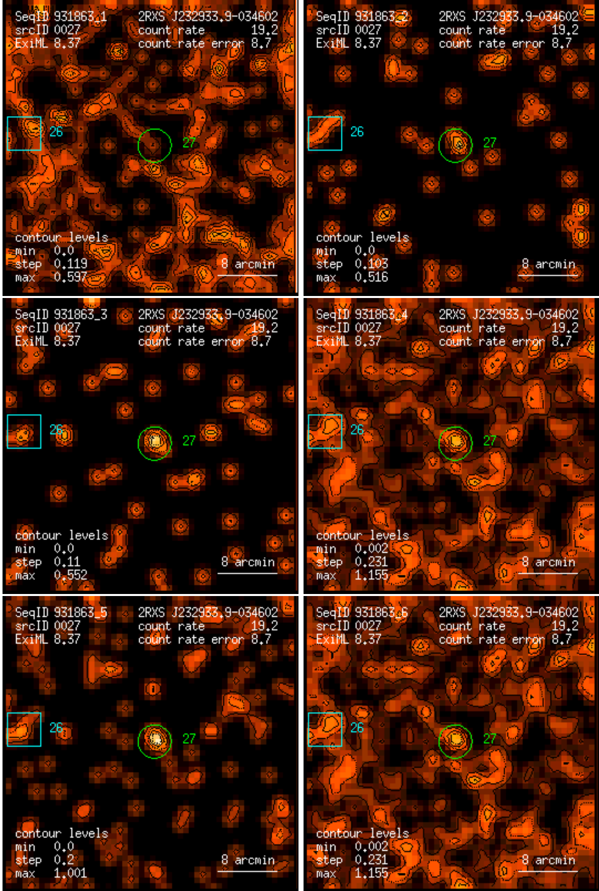
Figure 27: RASS 931863: detection 0027: band rate images, Gaussian filter: (1) PSPC channels 11 – 41, (2) 52 – 90, (3) 91 – 201, (4) 11 – 235, (5) 52 – 201, (6) 11 – 201. Broad band rates in counts/ks. Band rate contour levels in counts/ks/arcmin 2 .
