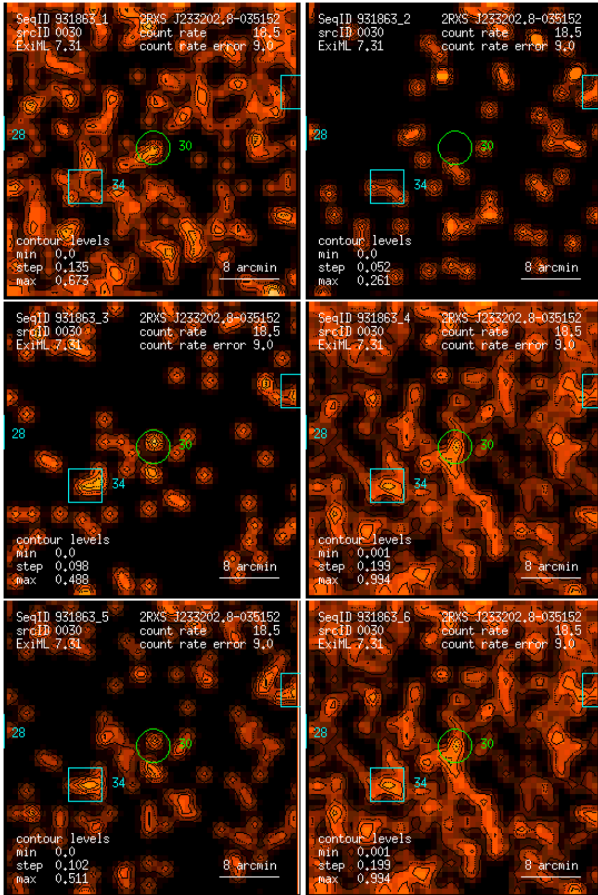
Figure 30: RASS 931863: detection 0030: band rate images, Gaussian filter: (1) PSPC channels 11 – 41, (2) 52 – 90, (3) 91 – 201, (4) 11 – 235, (5) 52 – 201, (6) 11 – 201. Broad band rates in counts/ks. Band rate contour levels in counts/ks/arcmin 2 .
