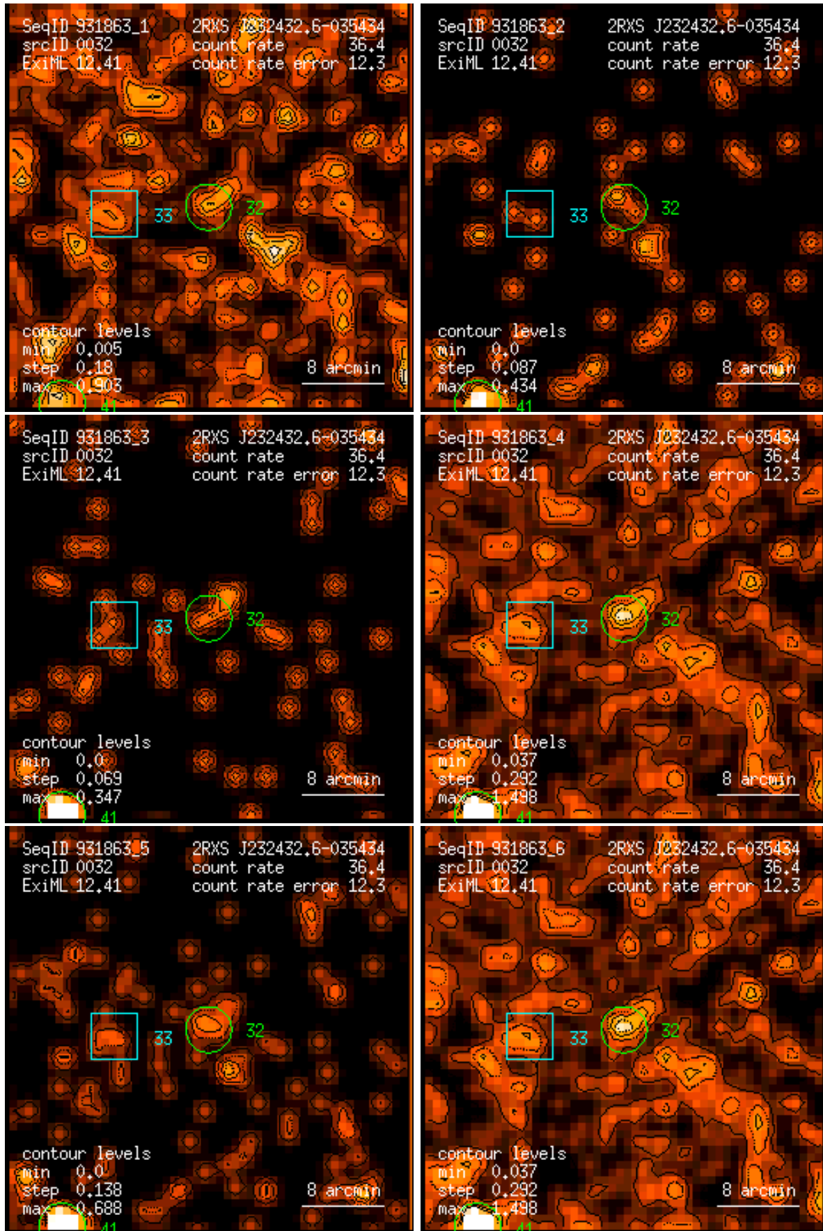
Figure 32: RASS 931863: detection 0032: band rate images, Gaussian filter: (1) PSPC channels 11 – 41, (2) 52 – 90, (3) 91 – 201, (4) 11 – 235, (5) 52 – 201, (6) 11 – 201. Broad band rates in counts/ks. Band rate contour levels in counts/ks/arcmin 2 .
