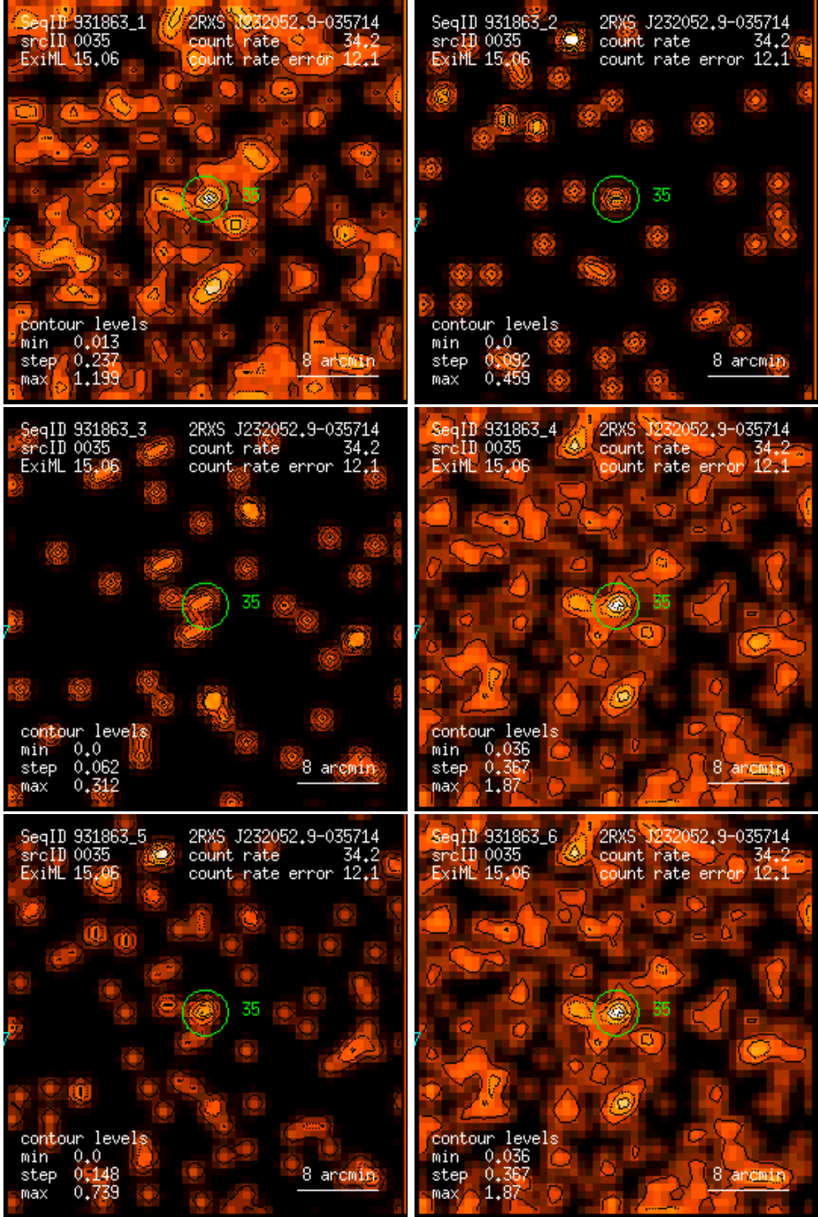
Figure 35: RASS 931863: detection 0035: band rate images, Gaussian filter: (1) PSPC channels 11 – 41, (2) 52 – 90, (3) 91 – 201, (4) 11 – 235, (5) 52 – 201, (6) 11 – 201. Broad band rates in counts/ks. Band rate contour levels in counts/ks/arcmin 2 .
