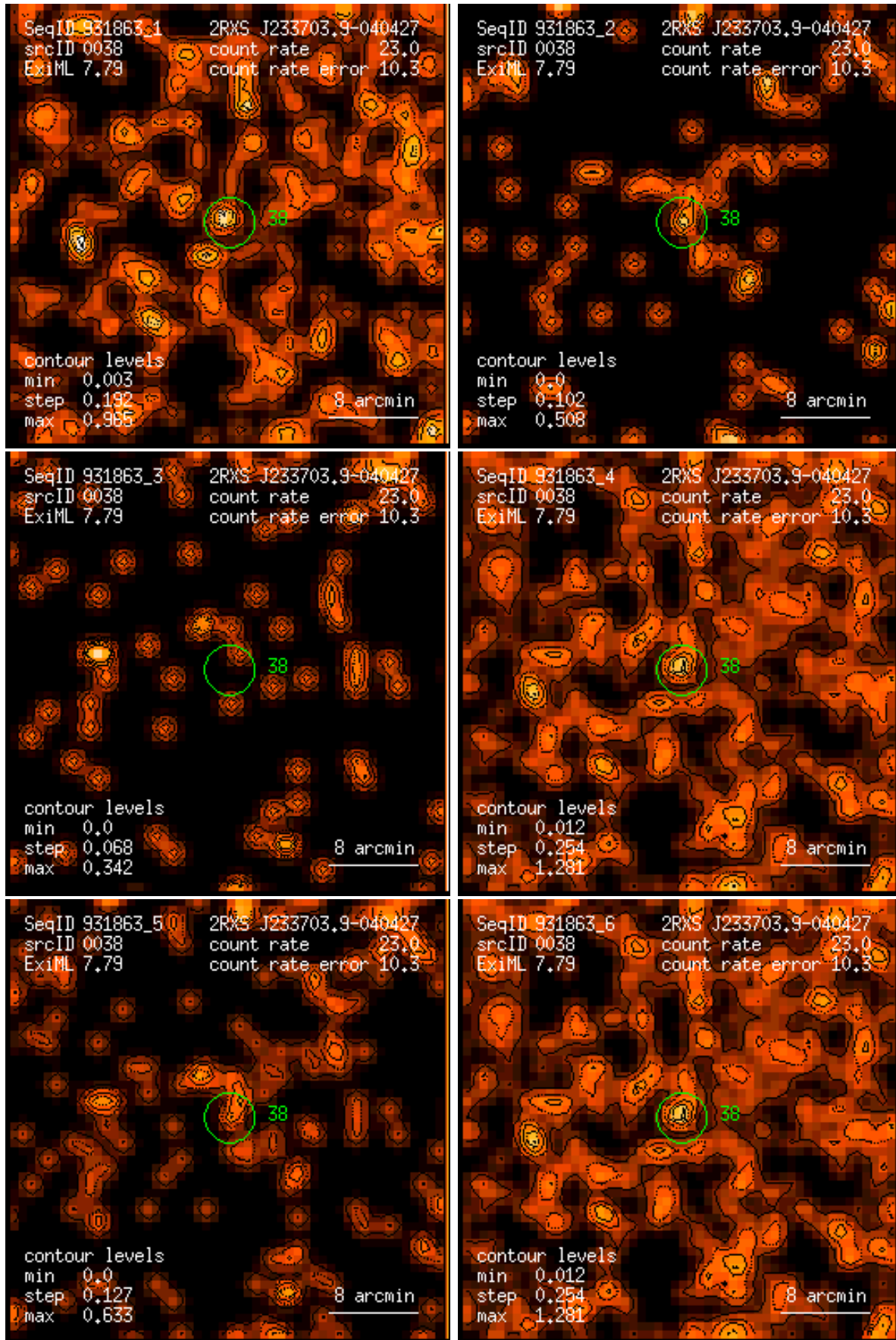
Figure 38: RASS 931863: detection 0038: band rate images, Gaussian filter: (1) PSPC channels 11 – 41, (2) 52 – 90, (3) 91 – 201, (4) 11 – 235, (5) 52 – 201, (6) 11 – 201. Broad band rates in counts/ks. Band rate contour levels in counts/ks/arcmin 2 .
