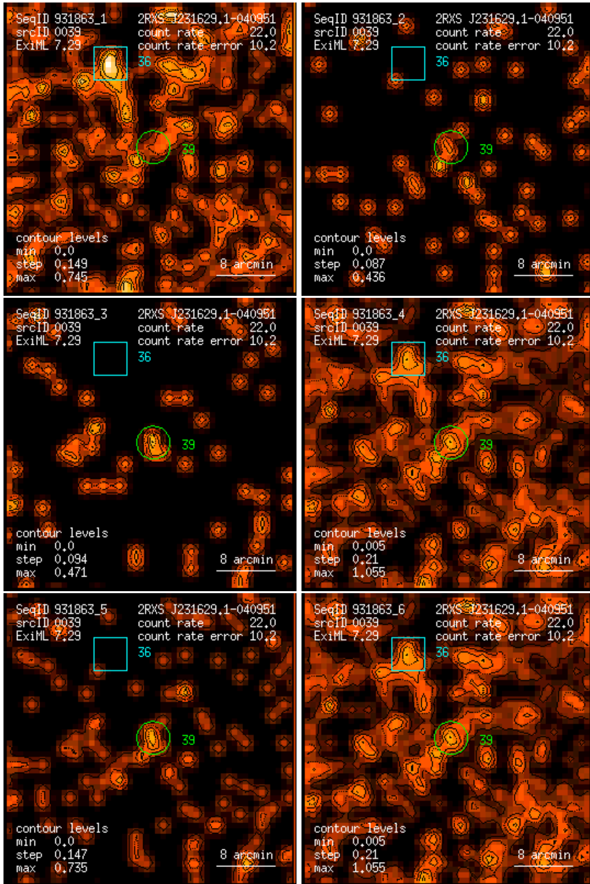
Figure 39: RASS 931863: detection 0039: band rate images, Gaussian filter: (1) PSPC channels 11 – 41, (2) 52 – 90, (3) 91 – 201, (4) 11 – 235, (5) 52 – 201, (6) 11 – 201. Broad band rates in counts/ks. Band rate contour levels in counts/ks/arcmin 2 .
