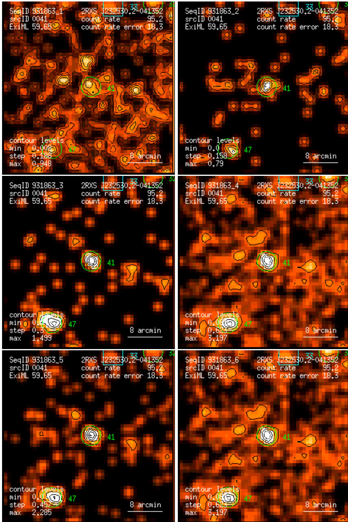
Figure 41: RASS 931863: detection 0041: band rate images, Gaussian filter: (1) PSPC channels 11 – 41, (2) 52 – 90, (3) 91 – 201, (4) 11 – 235, (5) 52 – 201, (6) 11 – 201. Broad band rates in counts/ks. Band rate contour levels in counts/ks/arcmin 2 .
