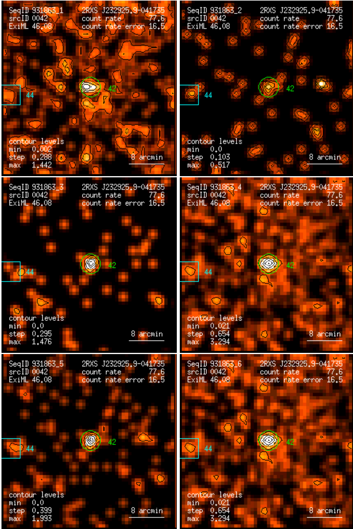
Figure 42: RASS 931863: detection 0042: band rate images, Gaussian filter: (1) PSPC channels 11 – 41, (2) 52 – 90, (3) 91 – 201, (4) 11 – 235, (5) 52 – 201, (6) 11 – 201. Broad band rates in counts/ks. Band rate contour levels in counts/ks/arcmin 2 .
