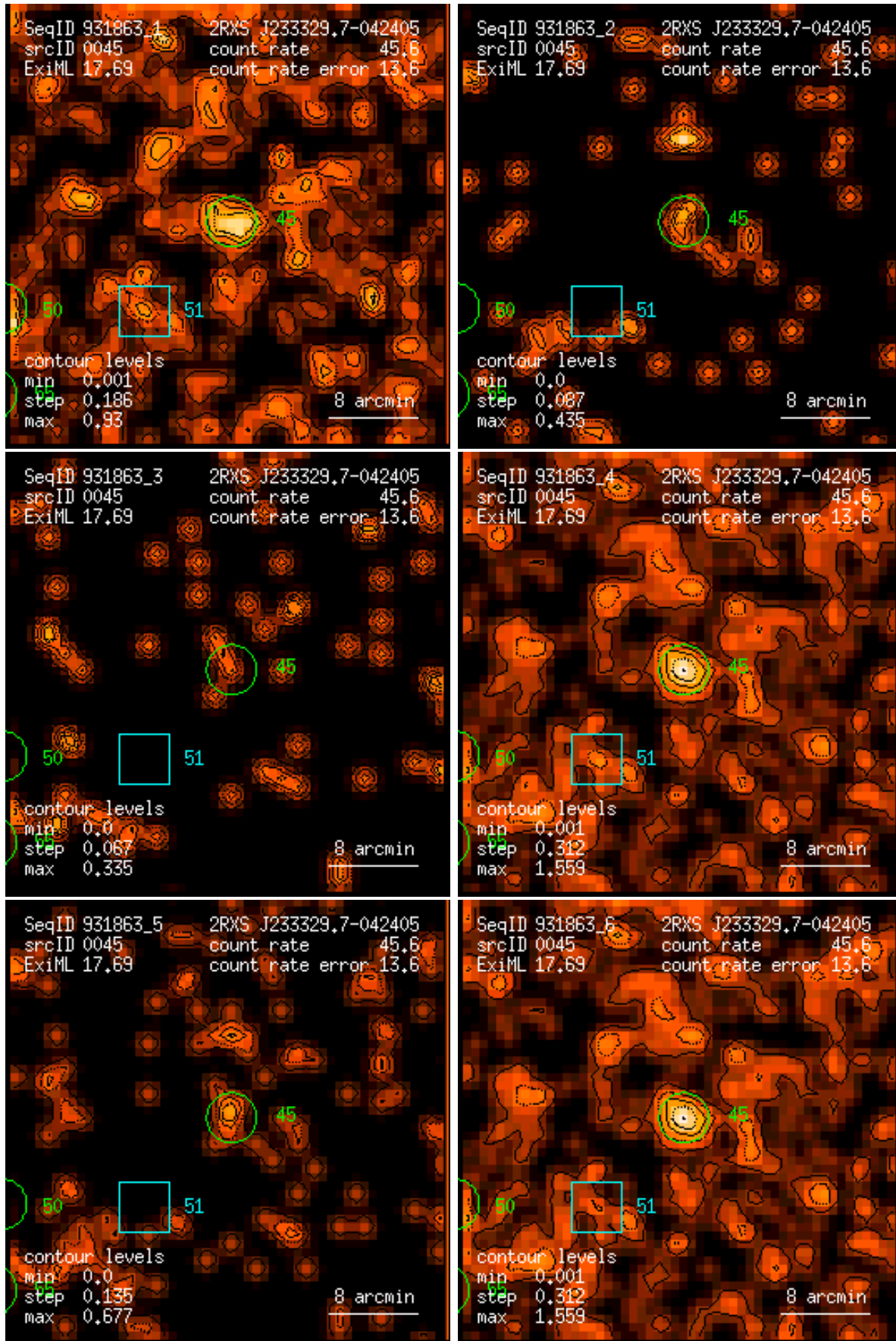
Figure 45: RASS 931863: detection 0045: band rate images, Gaussian filter: (1) PSPC channels 11 – 41, (2) 52 – 90, (3) 91 – 201, (4) 11 – 235, (5) 52 – 201, (6) 11 – 201. Broad band rates in counts/ks. Band rate contour levels in counts/ks/arcmin 2 .
