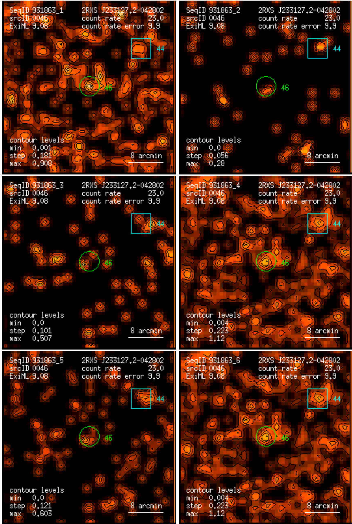
Figure 46: RASS 931863: detection 0046: band rate images, Gaussian filter: (1) PSPC channels 11 – 41, (2) 52 – 90, (3) 91 – 201, (4) 11 – 235, (5) 52 – 201, (6) 11 – 201. Broad band rates in counts/ks. Band rate contour levels in counts/ks/arcmin 2 .
