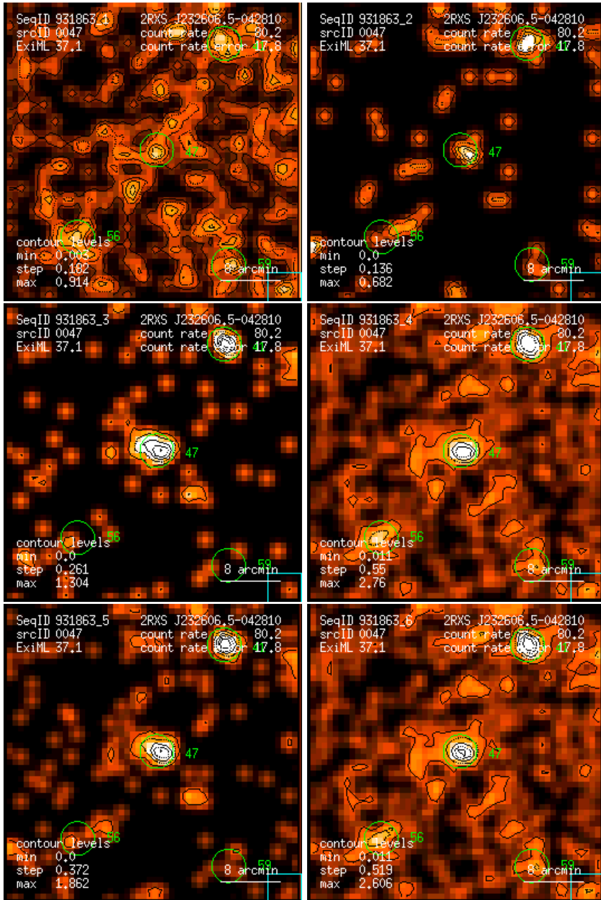
Figure 47: RASS 931863: detection 0047: band rate images, Gaussian filter: (1) PSPC channels 11 – 41, (2) 52 – 90, (3) 91 – 201, (4) 11 – 235, (5) 52 – 201, (6) 11 – 201. Broad band rates in counts/ks. Band rate contour levels in counts/ks/arcmin 2 .
