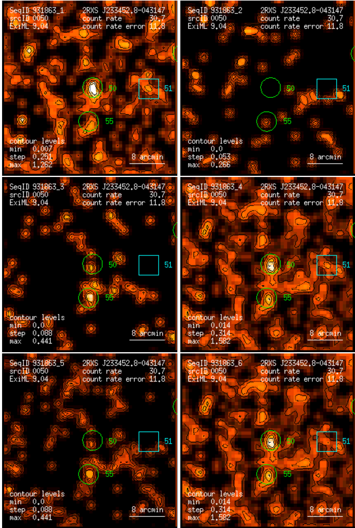
Figure 50: RASS 931863: detection 0050: band rate images, Gaussian filter: (1) PSPC channels 11 – 41, (2) 52 – 90, (3) 91 – 201, (4) 11 – 235, (5) 52 – 201, (6) 11 – 201. Broad band rates in counts/ks. Band rate contour levels in counts/ks/arcmin 2 .
