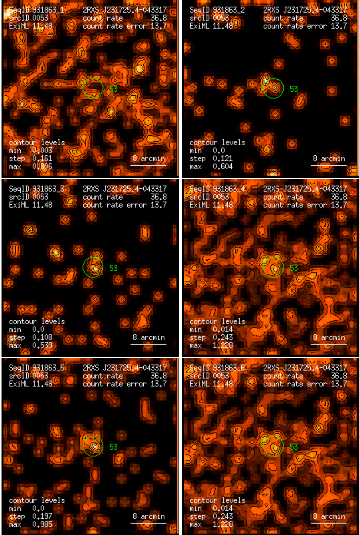
Figure 53: RASS 931863: detection 0053: band rate images, Gaussian filter: (1) PSPC channels 11 – 41, (2) 52 – 90, (3) 91 – 201, (4) 11 – 235, (5) 52 – 201, (6) 11 – 201. Broad band rates in counts/ks. Band rate contour levels in counts/ks/arcmin 2 .
