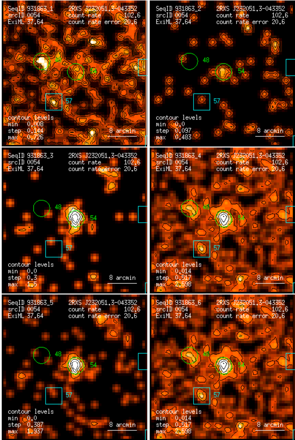
Figure 54: RASS 931863: detection 0054: band rate images, Gaussian filter: (1) PSPC channels 11 – 41, (2) 52 – 90, (3) 91 – 201, (4) 11 – 235, (5) 52 – 201, (6) 11 – 201. Broad band rates in counts/ks. Band rate contour levels in counts/ks/arcmin 2 .
