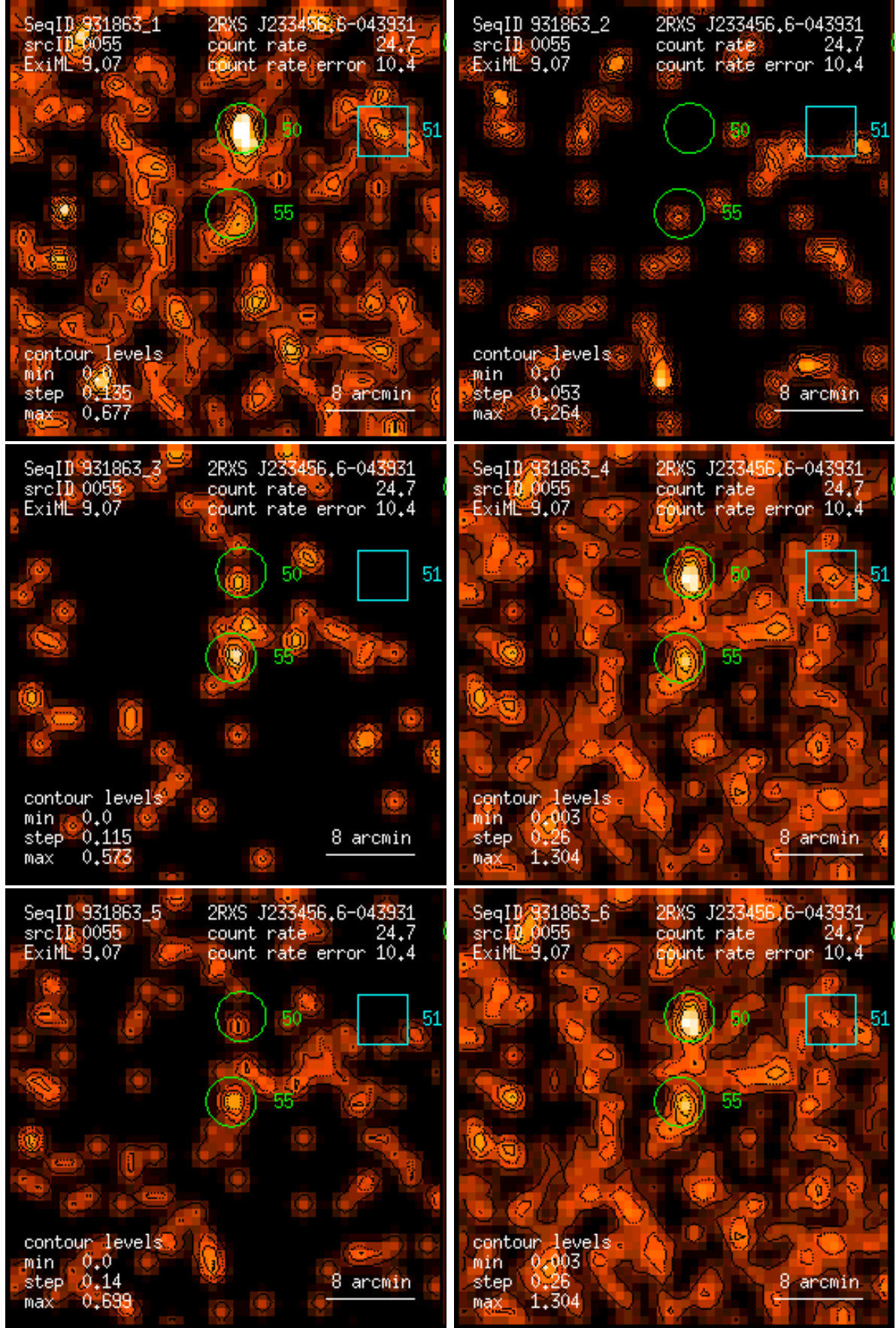
Figure 55: RASS 931863: detection 0055: band rate images, Gaussian filter: (1) PSPC channels 11 – 41, (2) 52 – 90, (3) 91 – 201, (4) 11 – 235, (5) 52 – 201, (6) 11 – 201. Broad band rates in counts/ks. Band rate contour levels in counts/ks/arcmin 2 .
