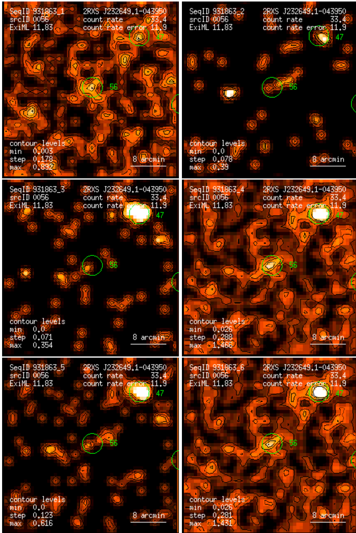
Figure 56: RASS 931863: detection 0056: band rate images, Gaussian filter: (1) PSPC channels 11 – 41, (2) 52 – 90, (3) 91 – 201, (4) 11 – 235, (5) 52 – 201, (6) 11 – 201. Broad band rates in counts/ks. Band rate contour levels in counts/ks/arcmin 2 .
