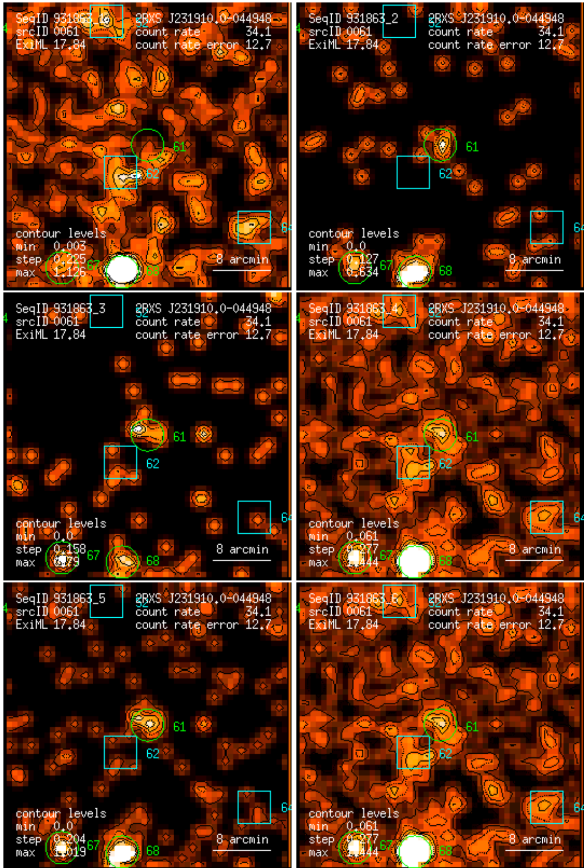
Figure 61: RASS 931863: detection 0061: band rate images, Gaussian filter: (1) PSPC channels 11 – 41, (2) 52 – 90, (3) 91 – 201, (4) 11 – 235, (5) 52 – 201, (6) 11 – 201. Broad band rates in counts/ks. Band rate contour levels in counts/ks/arcmin 2 .
