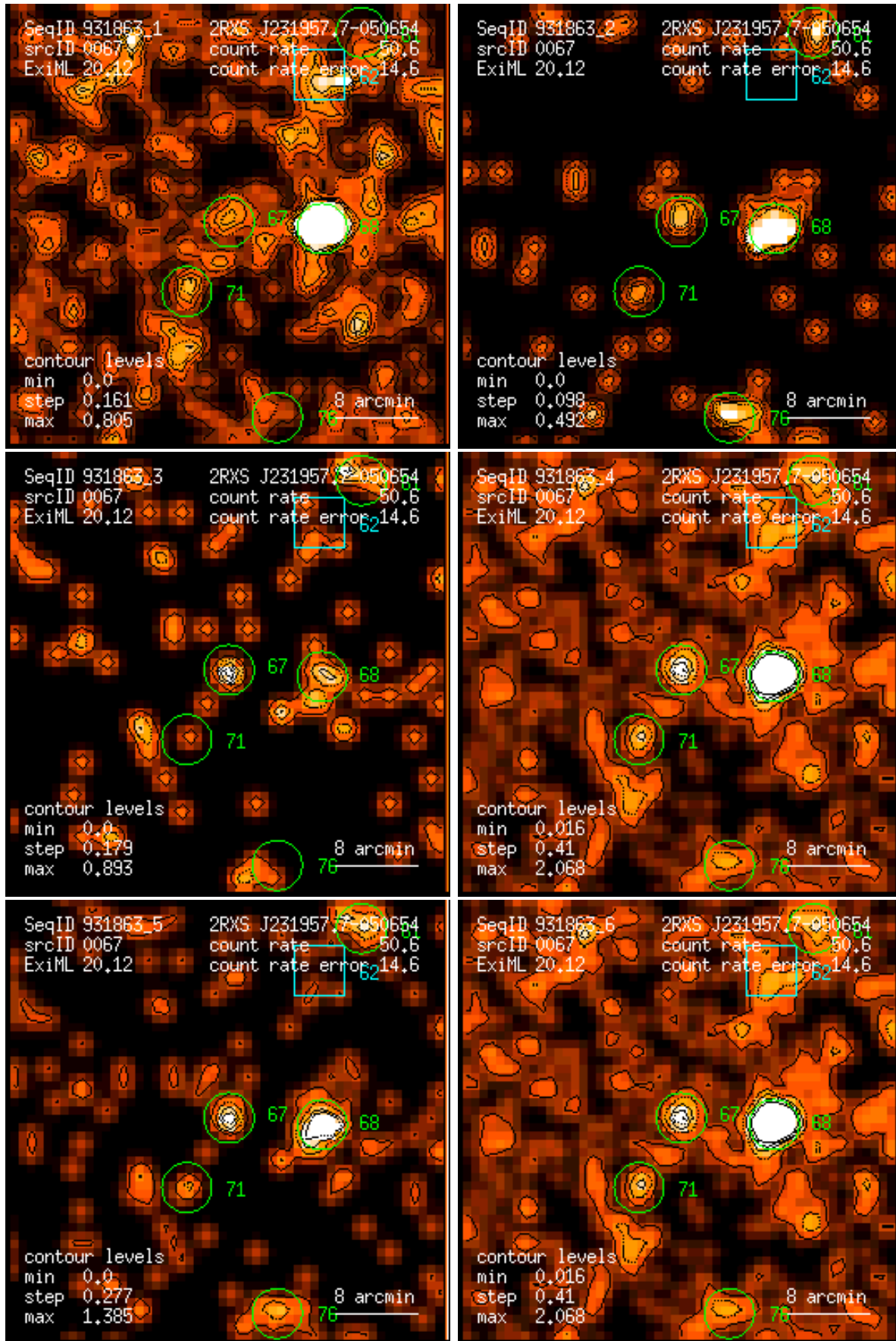
Figure 67: RASS 931863: detection 0067: band rate images, Gaussian filter: (1) PSPC channels 11 – 41, (2) 52 – 90, (3) 91 – 201, (4) 11 – 235, (5) 52 – 201, (6) 11 – 201. Broad band rates in counts/ks. Band rate contour levels in counts/ks/arcmin 2 .
