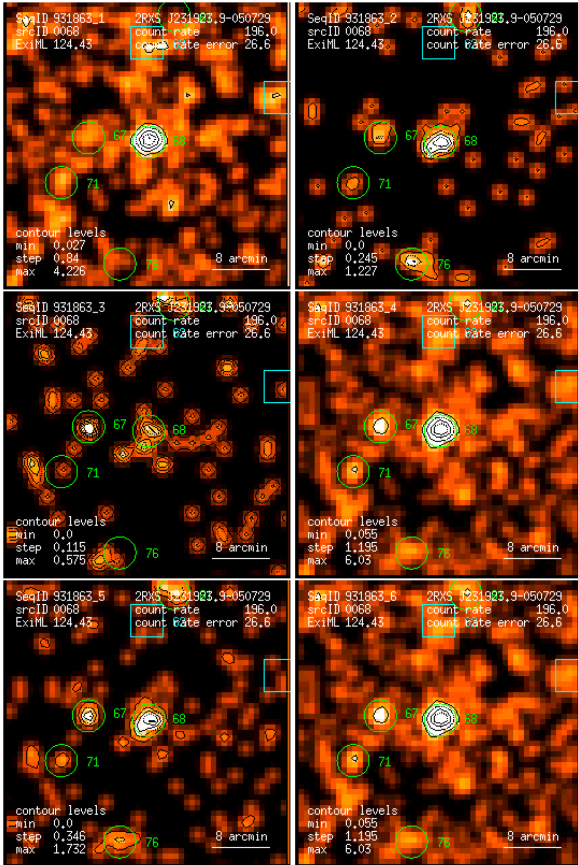
Figure 68: RASS 931863: detection 0068: band rate images, Gaussian filter: (1) PSPC channels 11 – 41, (2) 52 – 90, (3) 91 – 201, (4) 11 – 235, (5) 52 – 201, (6) 11 – 201. Broad band rates in counts/ks. Band rate contour levels in counts/ks/arcmin 2 .
