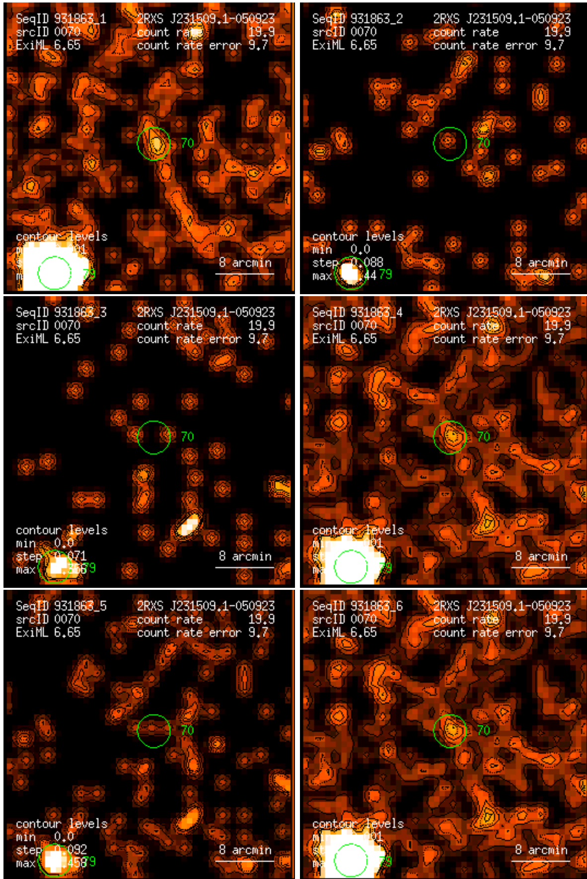
Figure 70: RASS 931863: detection 0070: band rate images, Gaussian filter: (1) PSPC channels 11 – 41, (2) 52 – 90, (3) 91 – 201, (4) 11 – 235, (5) 52 – 201, (6) 11 – 201. Broad band rates in counts/ks. Band rate contour levels in counts/ks/arcmin 2 .
