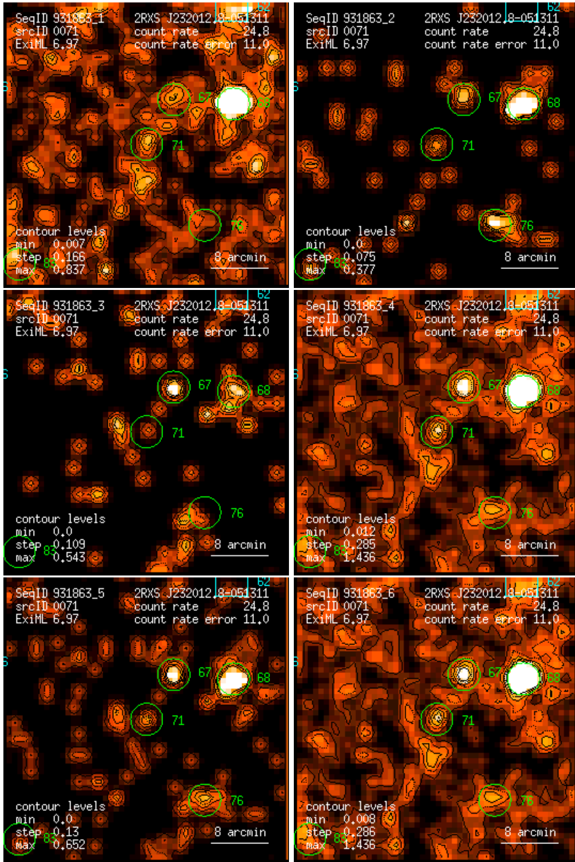
Figure 71: RASS 931863: detection 0071: band rate images, Gaussian filter: (1) PSPC channels 11 – 41, (2) 52 – 90, (3) 91 – 201, (4) 11 – 235, (5) 52 – 201, (6) 11 – 201. Broad band rates in counts/ks. Band rate contour levels in counts/ks/arcmin 2 .
