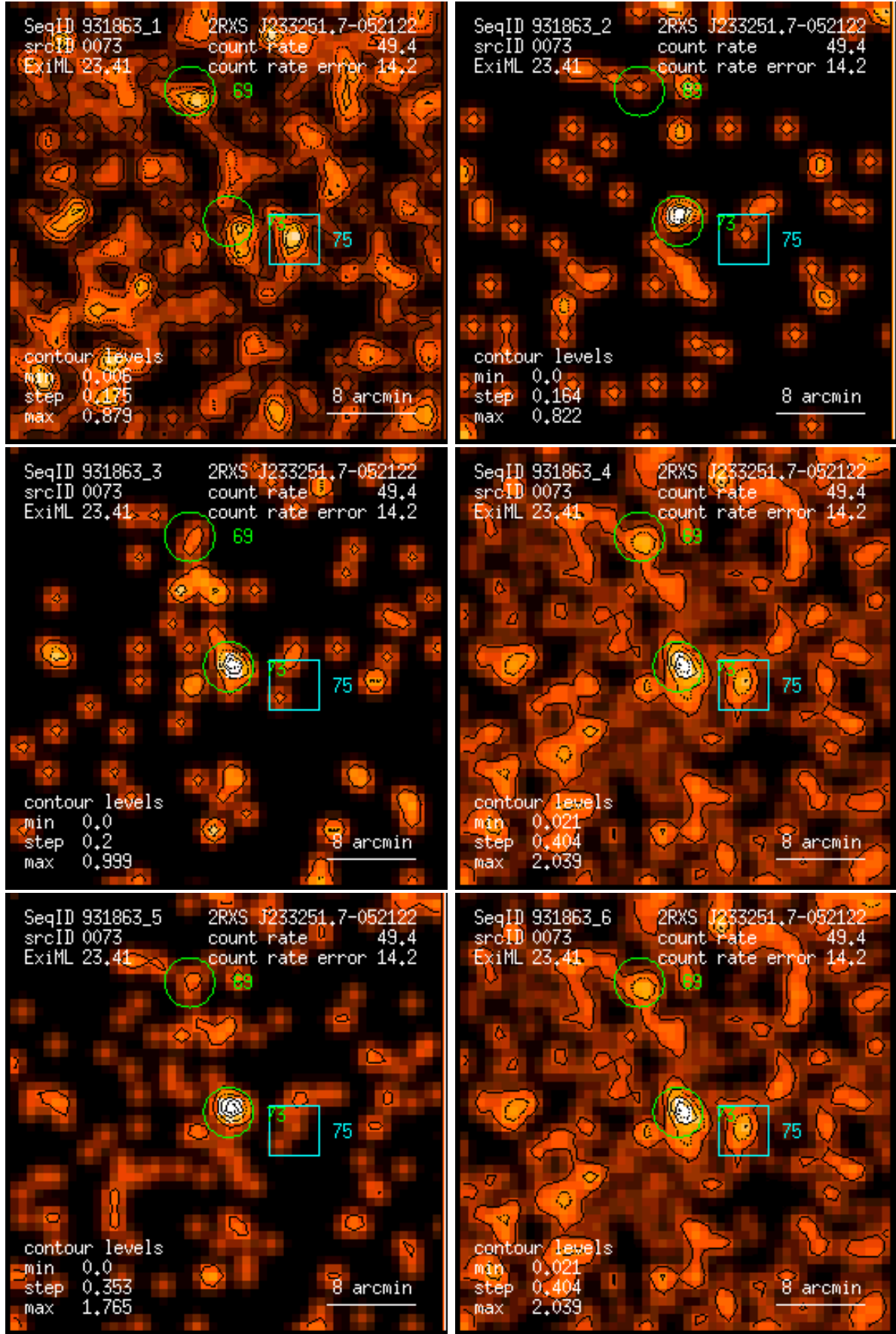
Figure 73: RASS 931863: detection 0073: band rate images, Gaussian filter: (1) PSPC channels 11 – 41, (2) 52 – 90, (3) 91 – 201, (4) 11 – 235, (5) 52 – 201, (6) 11 – 201. Broad band rates in counts/ks. Band rate contour levels in counts/ks/arcmin 2 .
