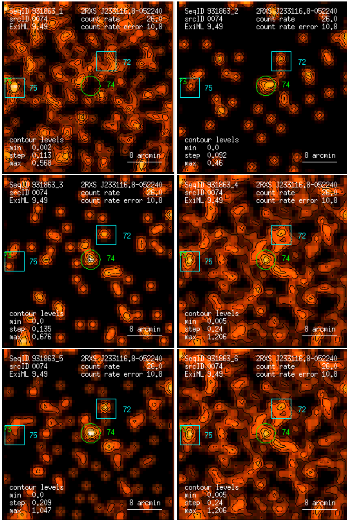
Figure 74: RASS 931863: detection 0074: band rate images, Gaussian filter: (1) PSPC channels 11 – 41, (2) 52 – 90, (3) 91 – 201, (4) 11 – 235, (5) 52 – 201, (6) 11 – 201. Broad band rates in counts/ks. Band rate contour levels in counts/ks/arcmin 2 .
