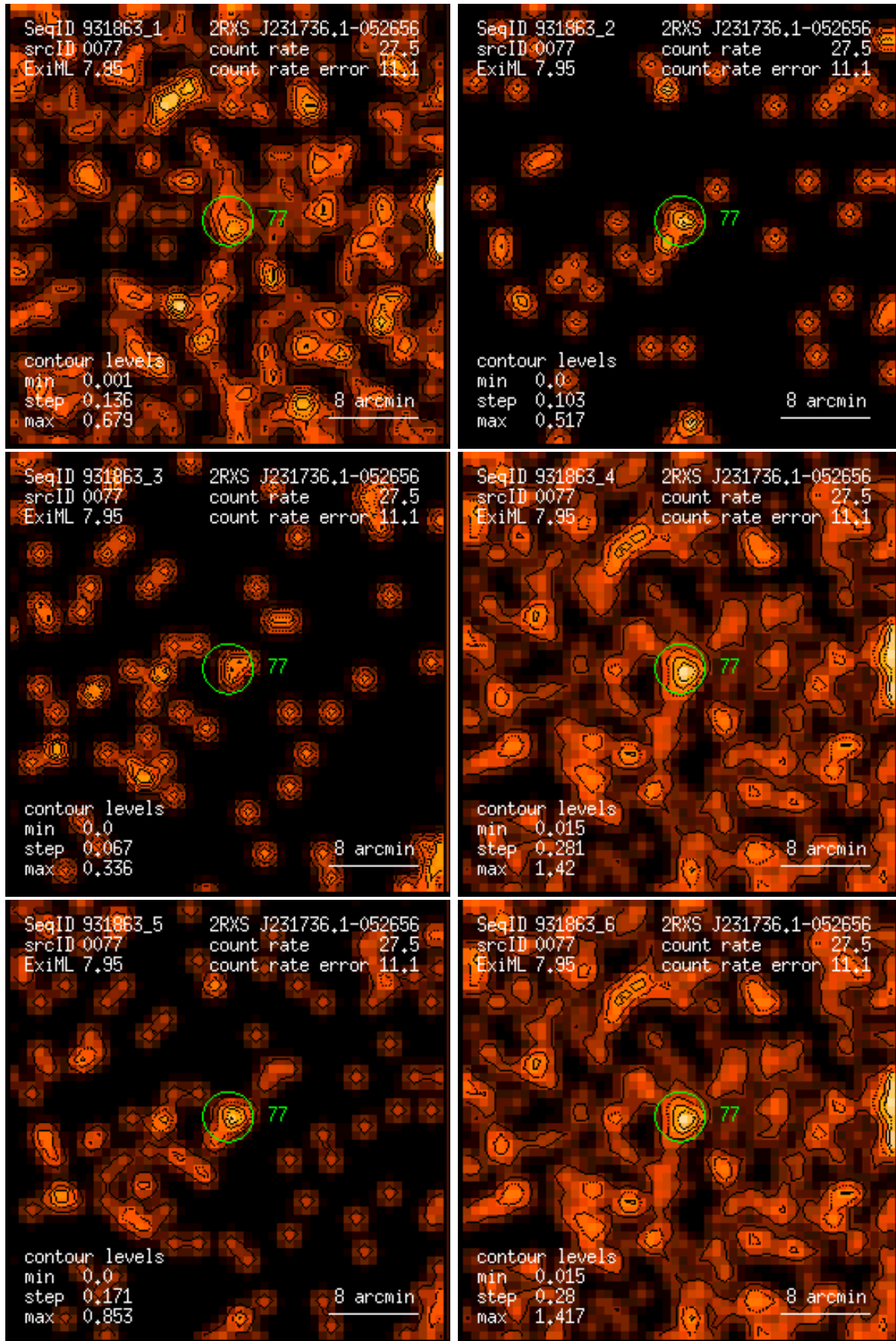
Figure 77: RASS 931863: detection 0077: band rate images, Gaussian filter: (1) PSPC channels 11 – 41, (2) 52 – 90, (3) 91 – 201, (4) 11 – 235, (5) 52 – 201, (6) 11 – 201. Broad band rates in counts/ks. Band rate contour levels in counts/ks/arcmin 2 .
