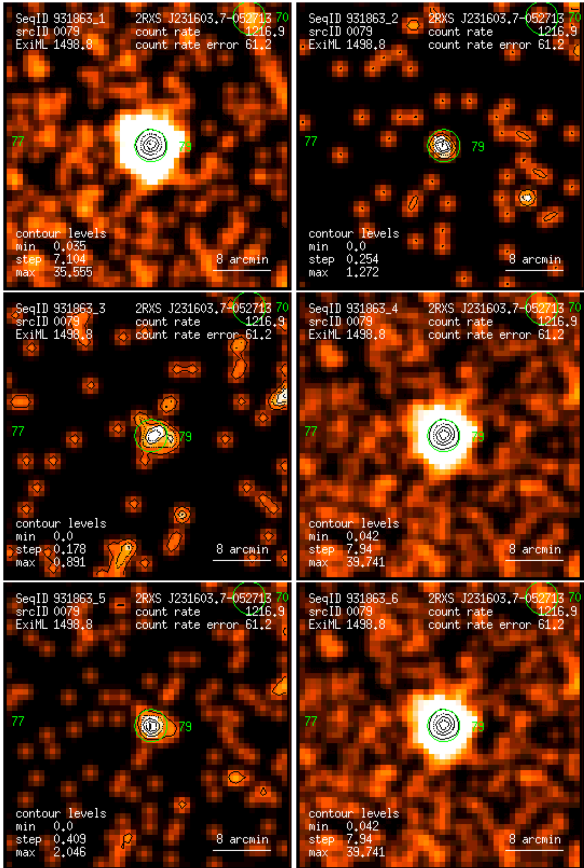
Figure 79: RASS 931863: detection 0079: band rate images, Gaussian filter: (1) PSPC channels 11 – 41, (2) 52 – 90, (3) 91 – 201, (4) 11 – 235, (5) 52 – 201, (6) 11 – 201. Broad band rates in counts/ks. Band rate contour levels in counts/ks/arcmin 2 .
