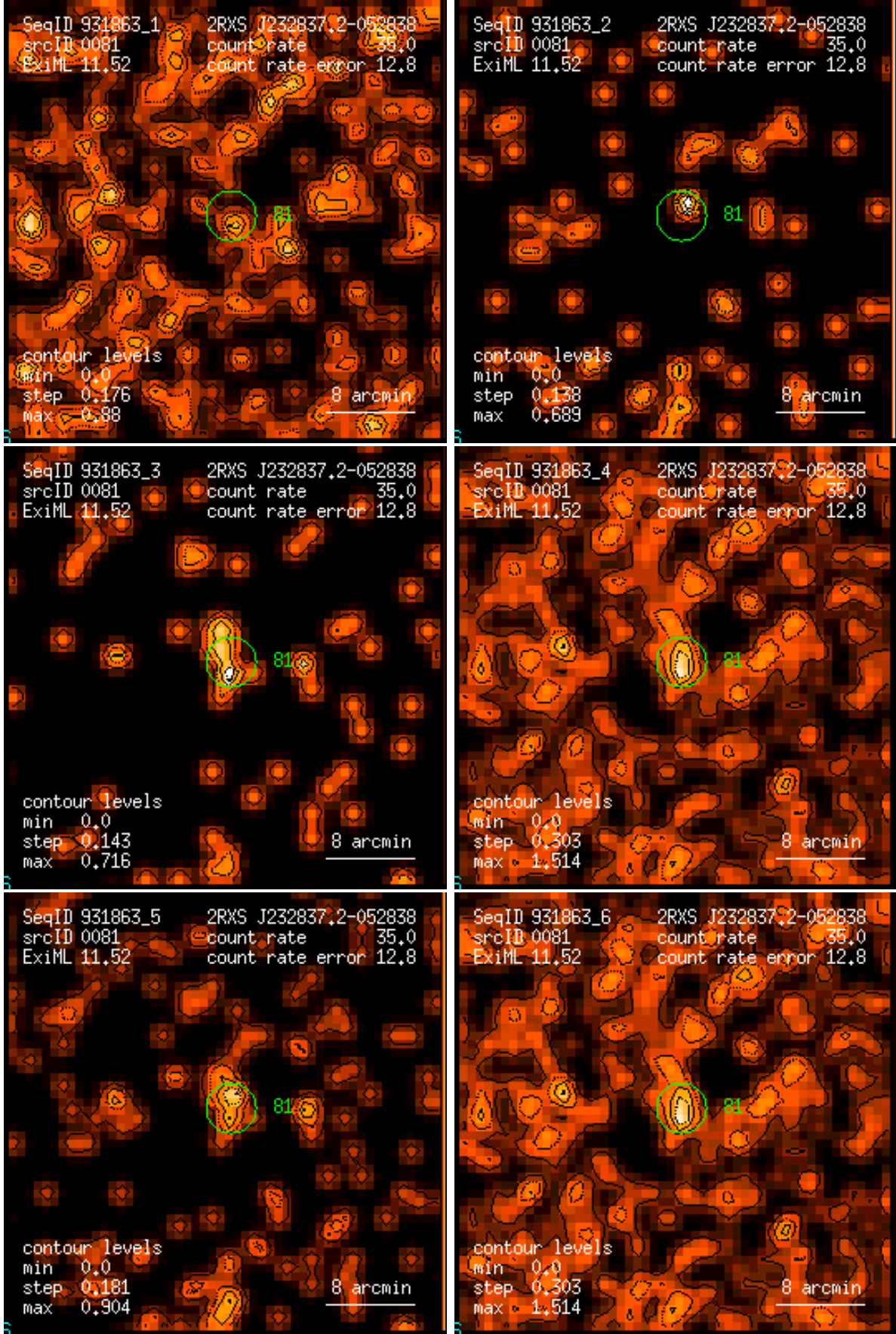
Figure 81: RASS 931863: detection 0081: band rate images, Gaussian filter: (1) PSPC channels 11 – 41, (2) 52 – 90, (3) 91 – 201, (4) 11 – 235, (5) 52 – 201, (6) 11 – 201. Broad band rates in counts/ks. Band rate contour levels in counts/ks/arcmin 2 .
