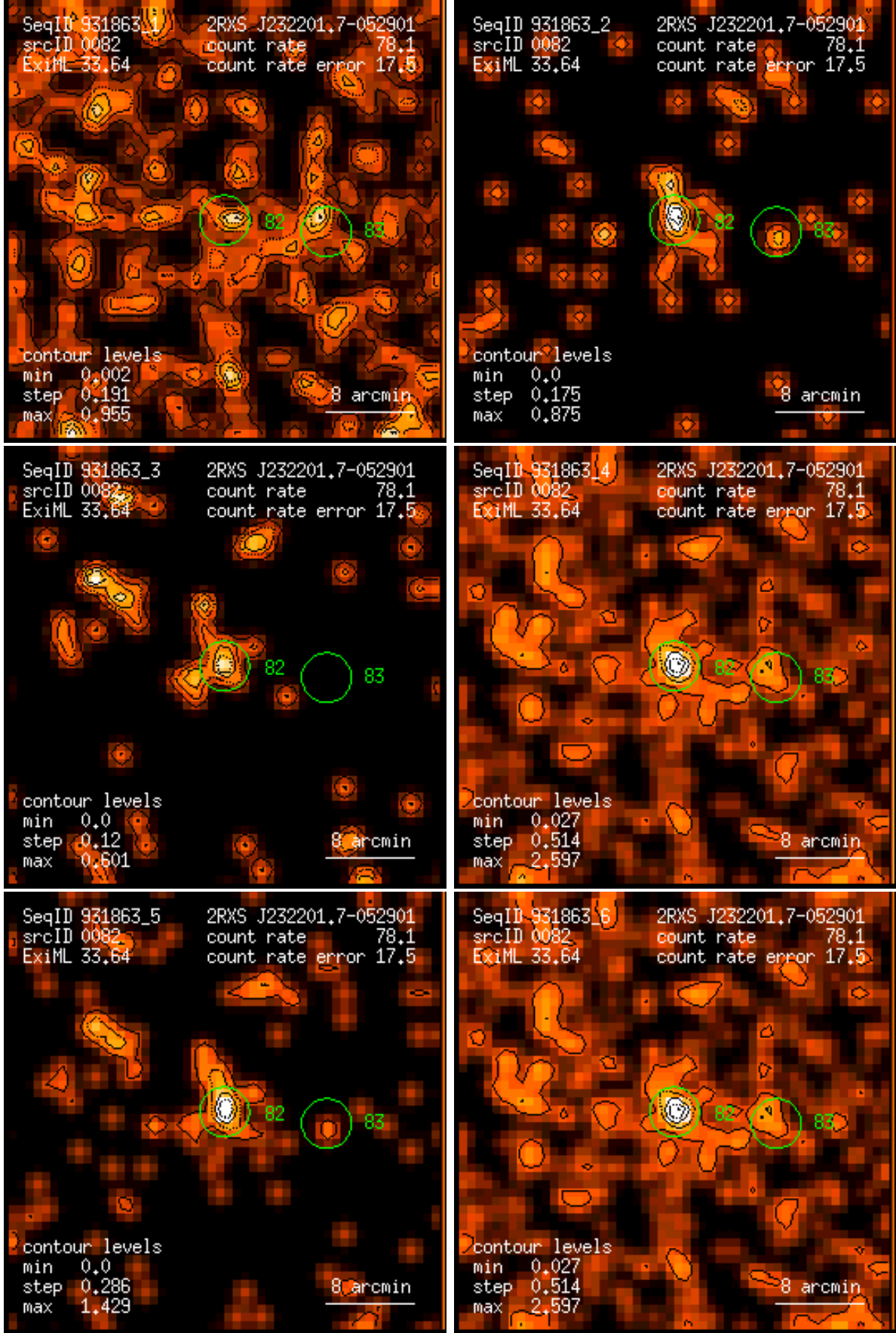
Figure 82: RASS 931863: detection 0082: band rate images, Gaussian filter: (1) PSPC channels 11 – 41, (2) 52 – 90, (3) 91 – 201, (4) 11 – 235, (5) 52 – 201, (6) 11 – 201. Broad band rates in counts/ks. Band rate contour levels in counts/ks/arcmin 2 .
