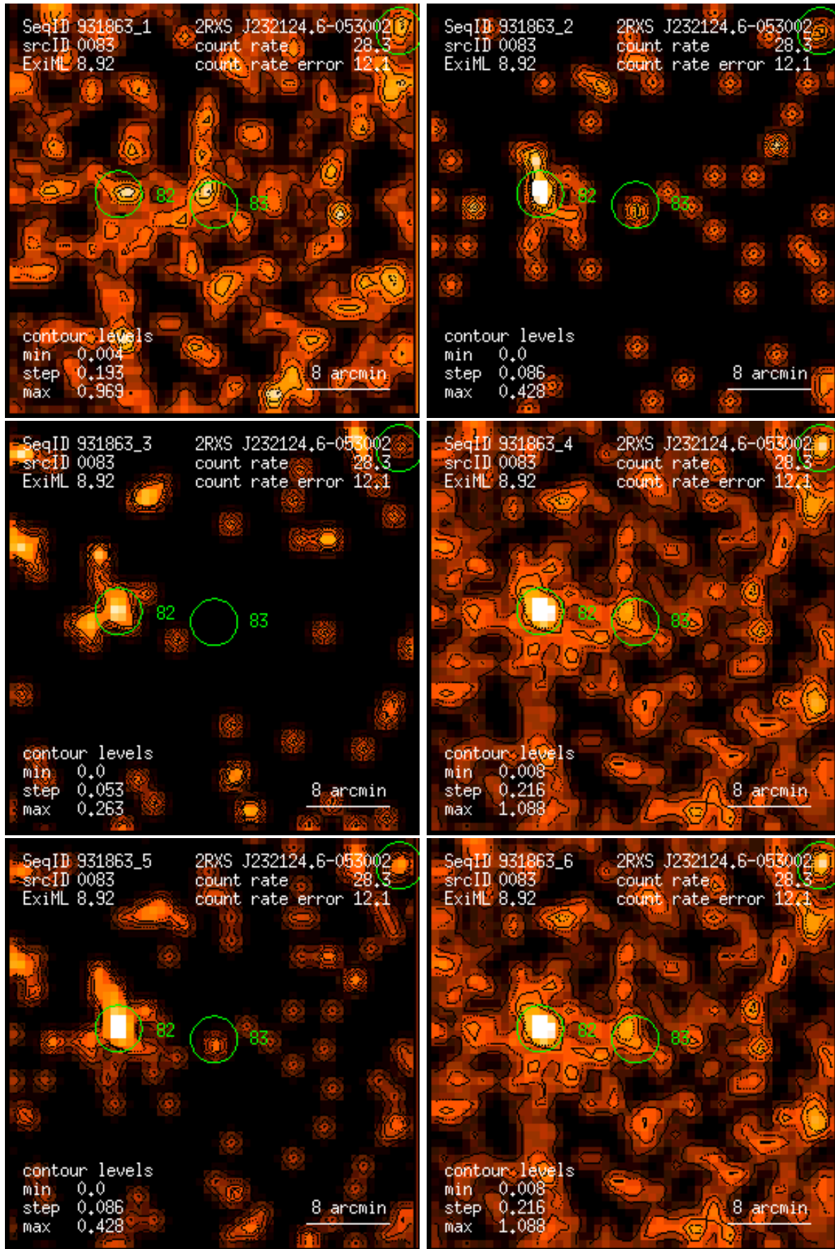
Figure 83: RASS 931863: detection 0083: band rate images, Gaussian filter: (1) PSPC channels 11 – 41, (2) 52 – 90, (3) 91 – 201, (4) 11 – 235, (5) 52 – 201, (6) 11 – 201. Broad band rates in counts/ks. Band rate contour levels in counts/ks/arcmin 2 .
