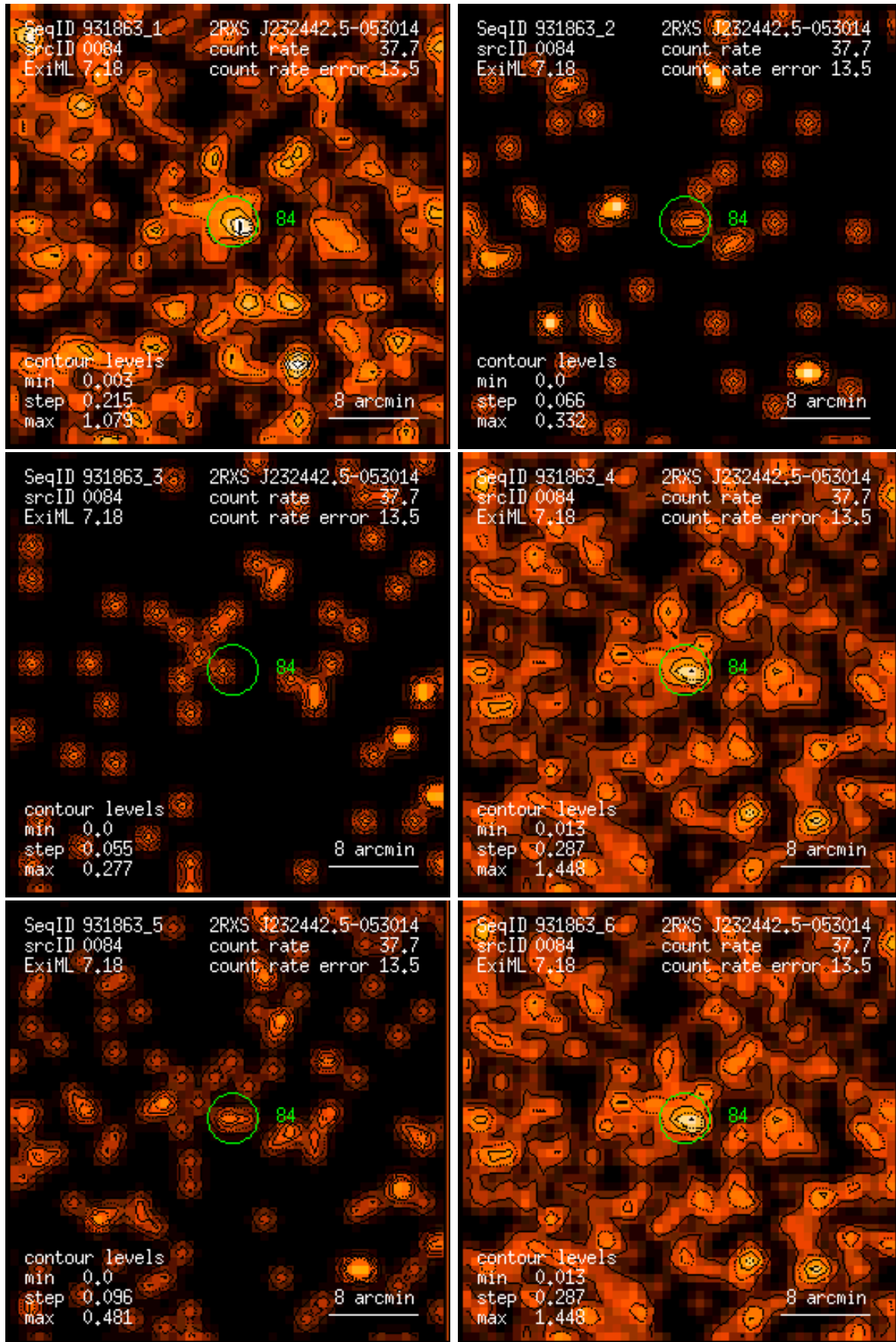
Figure 84: RASS 931863: detection 0084: band rate images, Gaussian filter: (1) PSPC channels 11 – 41, (2) 52 – 90, (3) 91 – 201, (4) 11 – 235, (5) 52 – 201, (6) 11 – 201. Broad band rates in counts/ks. Band rate contour levels in counts/ks/arcmin 2 .
