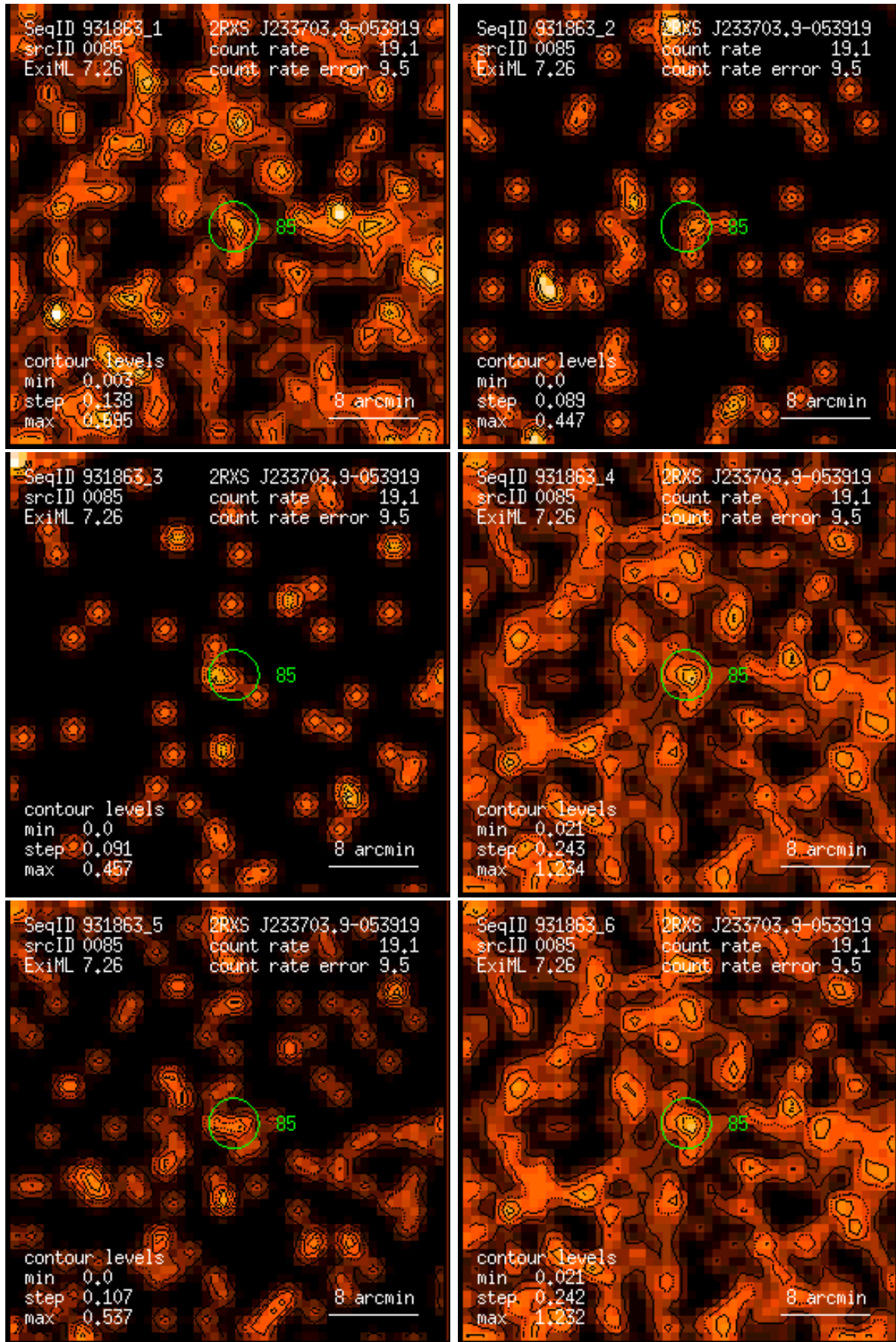
Figure 85: RASS 931863: detection 0085: band rate images, Gaussian filter: (1) PSPC channels 11 – 41, (2) 52 – 90, (3) 91 – 201, (4) 11 – 235, (5) 52 – 201, (6) 11 – 201. Broad band rates in counts/ks. Band rate contour levels in counts/ks/arcmin 2 .
