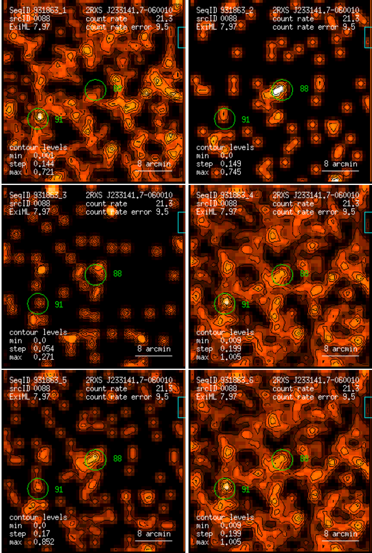
Figure 88: RASS 931863: detection 0088: band rate images, Gaussian filter: (1) PSPC channels 11 – 41, (2) 52 – 90, (3) 91 – 201, (4) 11 – 235, (5) 52 – 201, (6) 11 – 201. Broad band rates in counts/ks. Band rate contour levels in counts/ks/arcmin 2 .
