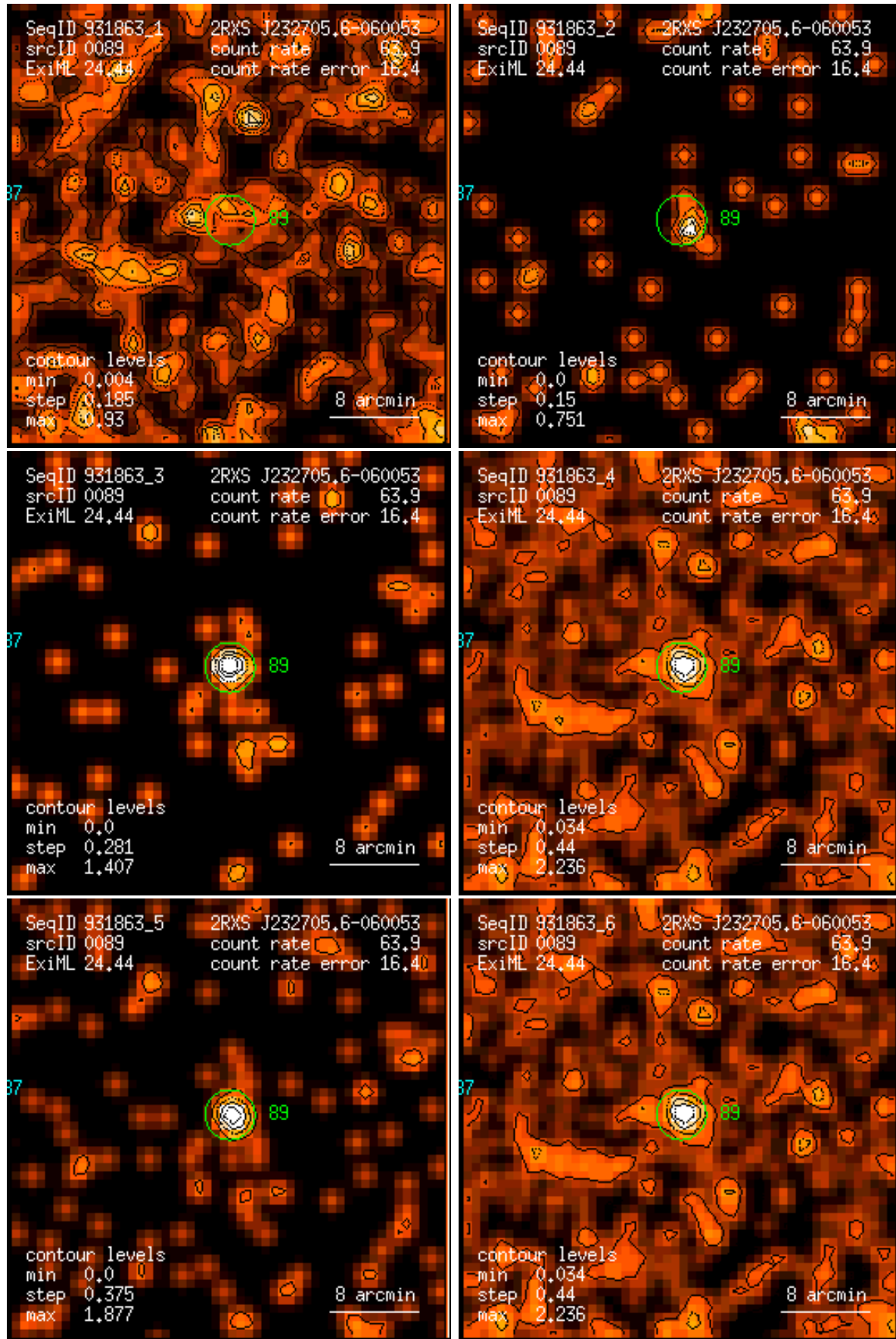
Figure 89: RASS 931863: detection 0089: band rate images, Gaussian filter: (1) PSPC channels 11 – 41, (2) 52 – 90, (3) 91 – 201, (4) 11 – 235, (5) 52 – 201, (6) 11 – 201. Broad band rates in counts/ks. Band rate contour levels in counts/ks/arcmin 2 .
