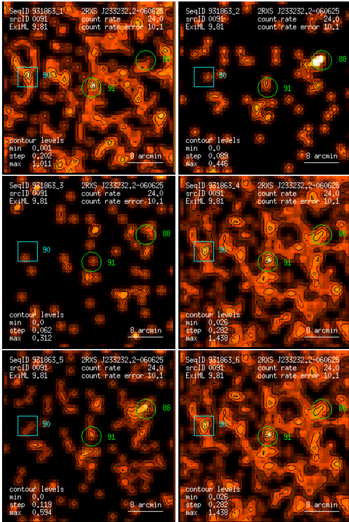
Figure 91: RASS 931863: detection 0091: band rate images, Gaussian filter: (1) PSPC channels 11 – 41, (2) 52 – 90, (3) 91 – 201, (4) 11 – 235, (5) 52 – 201, (6) 11 – 201. Broad band rates in counts/ks. Band rate contour levels in counts/ks/arcmin 2 .
