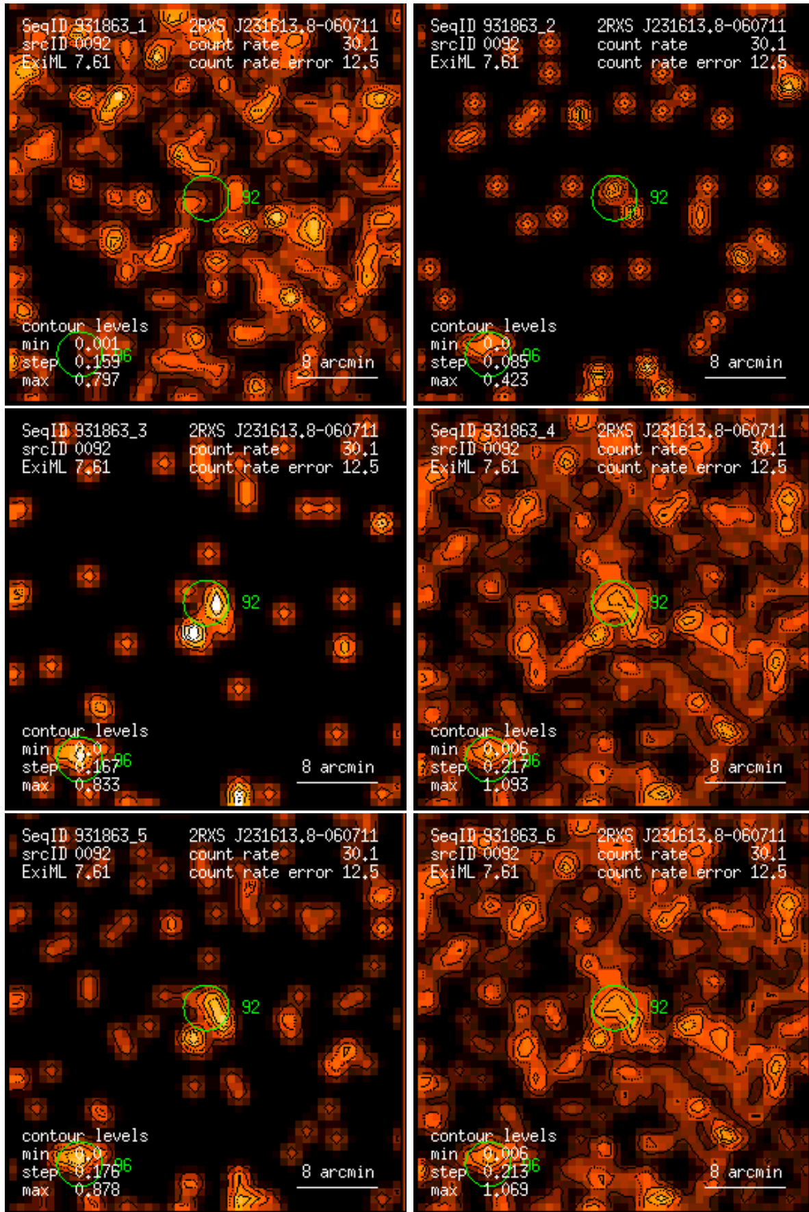
Figure 92: RASS 931863: detection 0092: band rate images, Gaussian filter: (1) PSPC channels 11 – 41, (2) 52 – 90, (3) 91 – 201, (4) 11 – 235, (5) 52 – 201, (6) 11 – 201. Broad band rates in counts/ks. Band rate contour levels in counts/ks/arcmin 2 .
