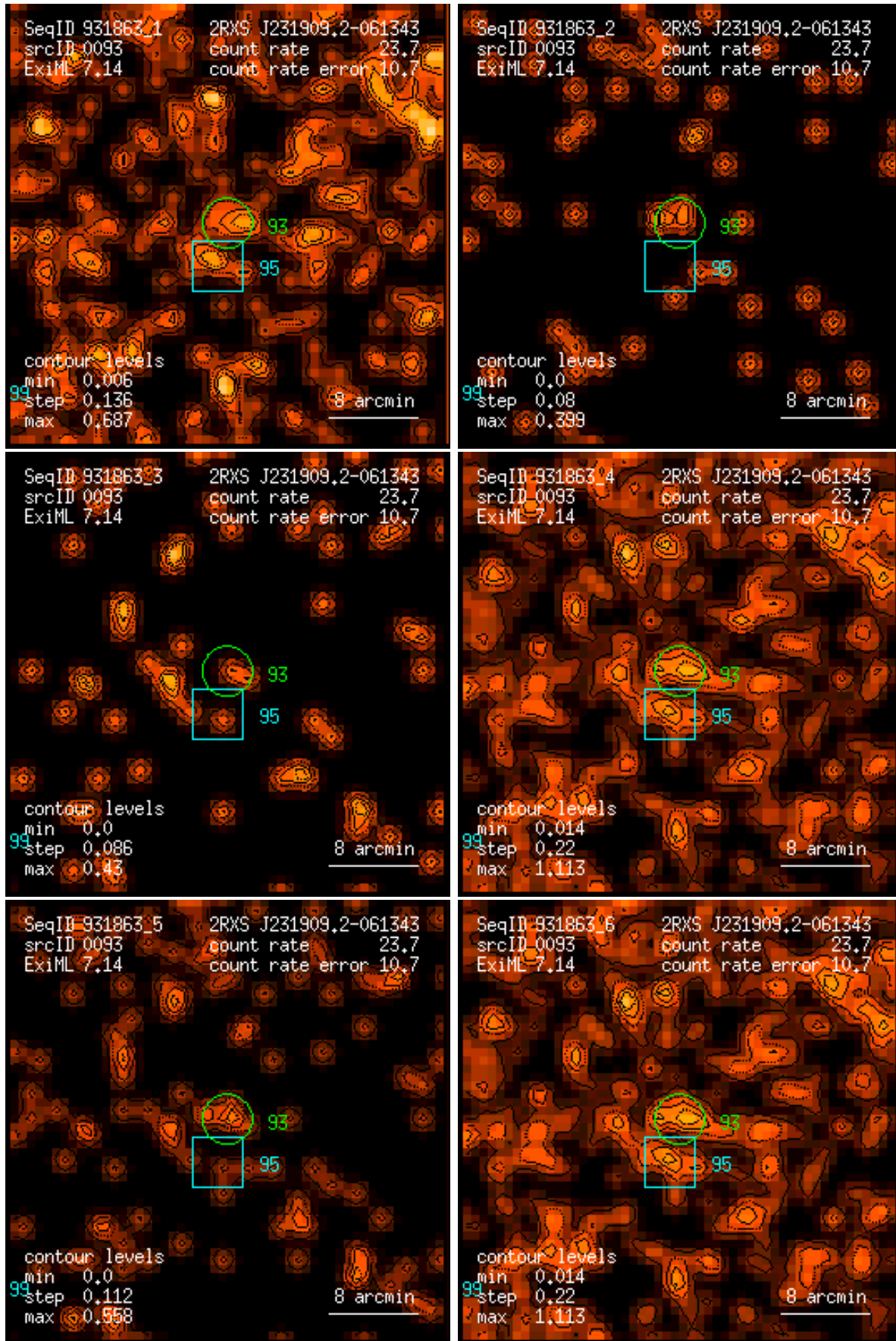
Figure 93: RASS 931863: detection 0093: band rate images, Gaussian filter: (1) PSPC channels 11 – 41, (2) 52 – 90, (3) 91 – 201, (4) 11 – 235, (5) 52 – 201, (6) 11 – 201. Broad band rates in counts/ks. Band rate contour levels in counts/ks/arcmin 2 .
