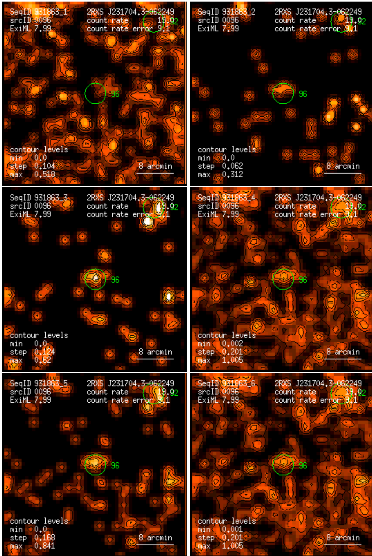
Figure 96: RASS 931863: detection 0096: band rate images, Gaussian filter: (1) PSPC channels 11 – 41, (2) 52 – 90, (3) 91 – 201, (4) 11 – 235, (5) 52 – 201, (6) 11 – 201. Broad band rates in counts/ks. Band rate contour levels in counts/ks/arcmin 2 .
