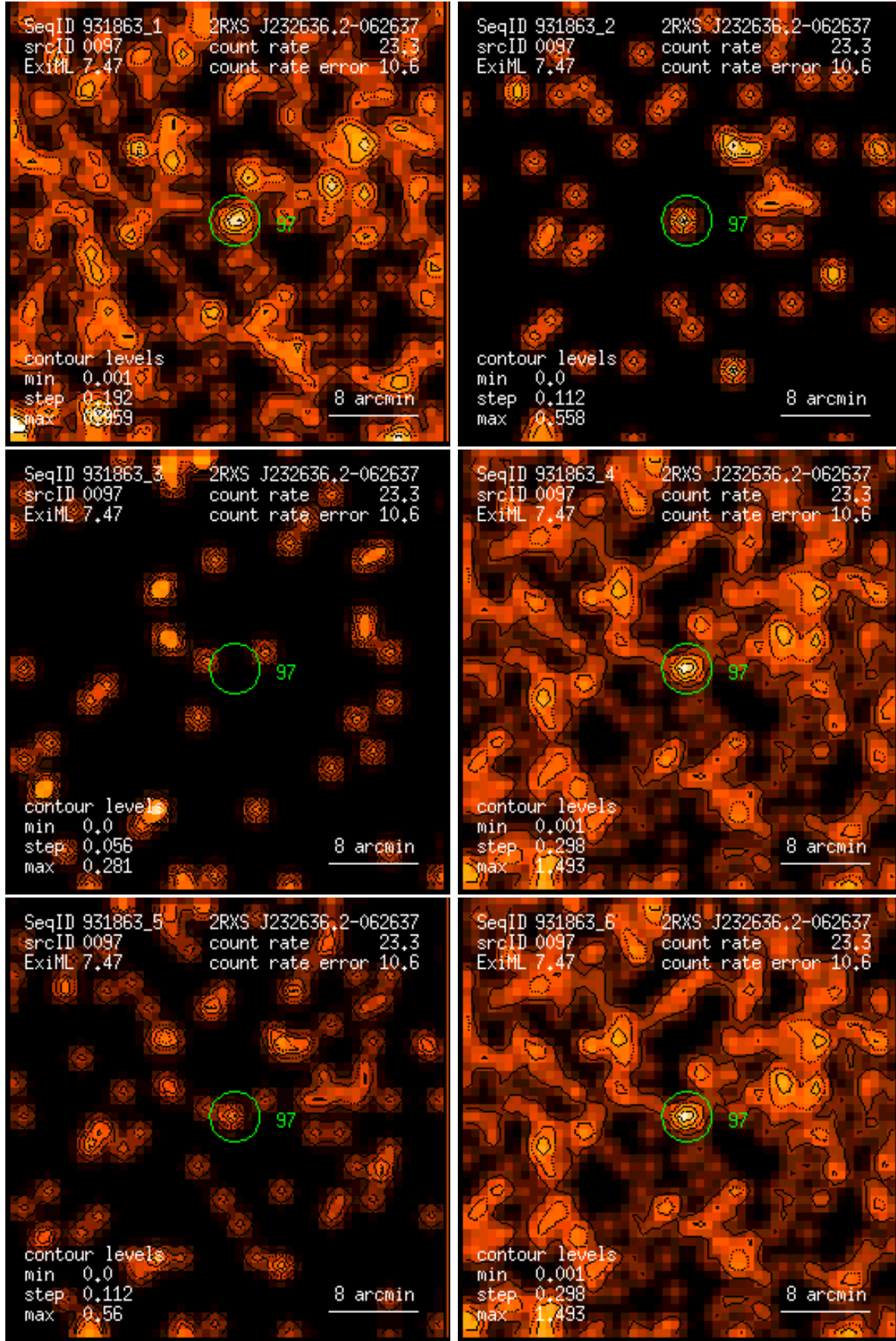
Figure 97: RASS 931863: detection 0097: band rate images, Gaussian filter: (1) PSPC channels 11 – 41, (2) 52 – 90, (3) 91 – 201, (4) 11 – 235, (5) 52 – 201, (6) 11 – 201. Broad band rates in counts/ks. Band rate contour levels in counts/ks/arcmin 2 .
