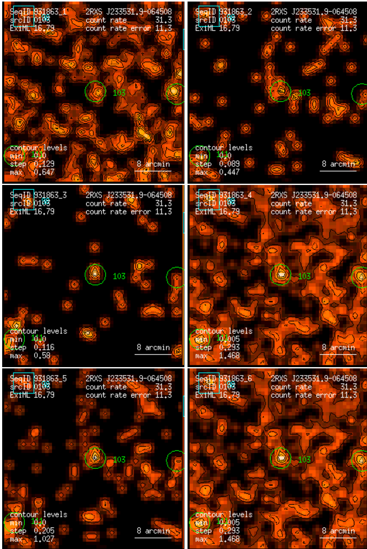
Figure 103: RASS 931863: detection 0103: band rate images, Gaussian filter: (1) PSPC channels 11 – 41, (2) 52 – 90, (3) 91 – 201, (4) 11 – 235, (5) 52 – 201, (6) 11 – 201. Broad band rates in counts/ks. Band rate contour levels in counts/ks/arcmin 2 .
